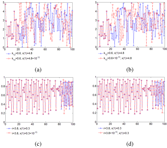
FIGURE 3. The MPSNC is more sensitivity to the initial value and the control parameters than the Logistical maps. (a) Sensitivity of MPSNC to x(1) ; (b) Sensitivity of MPSNC to k_{12} ; (c) Sensitivity of the Logistical map to x(1) ; (d) Sensitivity of the Logistical map to r .
