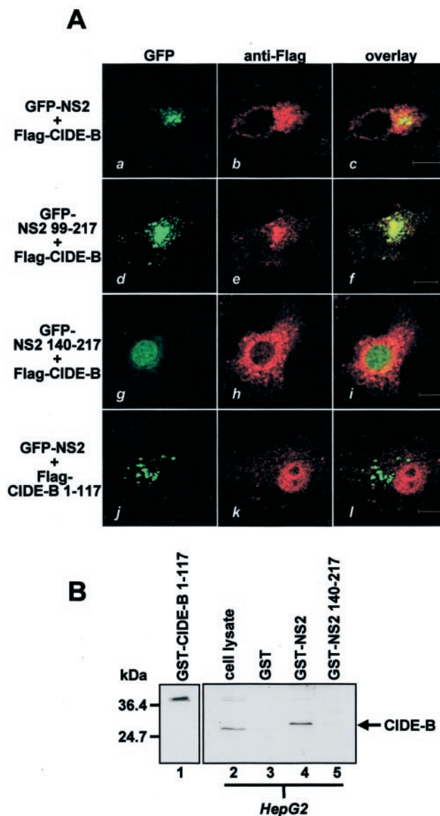
FIG. 4. NS2 associates with CIDE-B in the cell. A, HeLa cells were cotransfected with 12 \mu\text{g} of pcDNA3-FLAG-CIDE-B or pcDNA3-FLAG-CIDE-B(1–117) along with 12 \mu\text{g} of the different GFP vectors (panels a, d, g, and j). After 24 h, cells were fixed, permeabilized, treated with anti-FLAG monoclonal antibody, and stained with a Texas Red-conjugated Fab fragment recognizing mouse IgG. Subcellular localization of GFP proteins (panels a, d, g, and j) and FLAG-tagged proteins (panels b, e, h, and k) was analyzed by confocal microscopy, and colocalization was visualized by overlay (panels c, f, i, and l). B, shown is the binding of NS2 to endogenous CIDE-B. HepG2 lysates were incubated with equal amounts of purified GST (lane 3), GST-NS2 (lane 4), and GST-NS2(140–217) (lane 5). Bound proteins were resolved by SDS-PAGE, and CIDE-B association was analyzed by Western blotting. Purified GST-CIDE-B(1–117) (lane 1) and crude cell lysate (lane 2) were used as controls for specific anti-CIDE-B antibody recognition. Scale bar, 10 \mu\text{m} .
