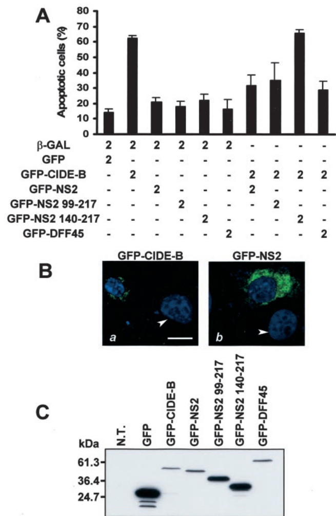
FIG. 5. The NS2 protein inhibits CIDE-B-induced apoptosis. A, quantification of apoptotic GFP-positive adherent cells. HeLa cells were cotransfected with the indicated amounts (0 or 2 \mu g) of different mammalian expression vectors. After 24 h, cells were stained with Hoechst 33342 and observed under a fluorescence microscope. Apoptotic GFP-expressing cells with condensed nuclei and fragmented chromatin were counted, and the percentage of cell death was calculated against the total number of GFP-positive cells ( n = 150 ). Error bars represent means \pm S.D. of three independent experiments. B, nuclear morphological analysis of GFP-positive adherent cells. HeLa cells were treated as described for A. The nuclear morphology of non-transfected non-apoptotic cells is indicated by white arrows. Scale bar = 10 \mu m (magnification \times 800 ). C, Western blot analysis. Lysates from cells expressing the indicated GFP fusion proteins were analyzed using anti-GFP antibody. \beta -GAL, \beta -galactosidase; N.T., non-transfected cells.
