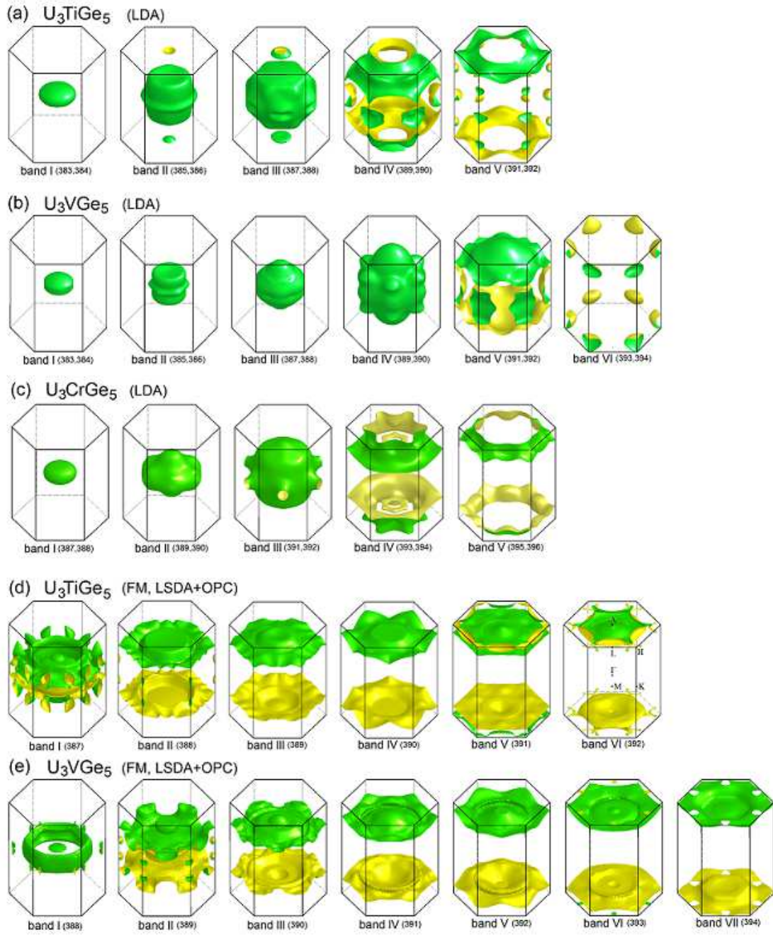
Fig. 10 Fermi surface sheets of non-magnetic (LDA) states for \text{U}_3\text{TiGe}_5 (a), \text{U}_3\text{VGe}_5 (b) and \text{U}_3\text{CrGe}_5 (c) originating from Kramers double-degenerate bands as well as of ferromagnetic (LSDA+OPC) states for \text{U}_3\text{TiGe}_5 (d) and \text{U}_3\text{VGe}_5 (e) coming from Kramers non-degenerate bands. The FS sheets are drawn separately within the hexagonal BZ boundaries. Green (dark) and yellow (light) sides of the surfaces adjoin electron and hole states, respectively.
