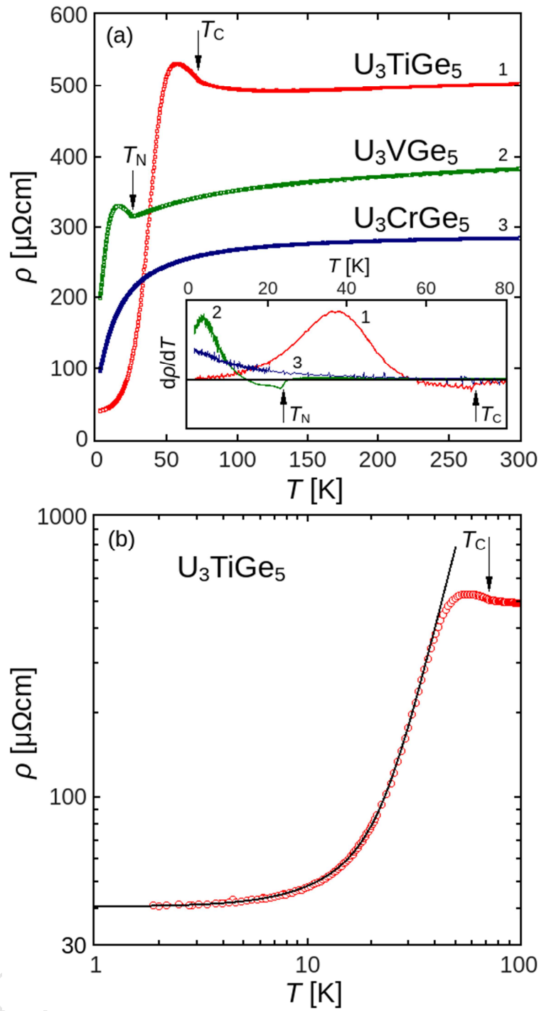
Fig. 6 (a) Temperature variation of electrical resistivity \rho(T) of \text{U}_3\text{TiGe}_5 , \text{U}_3\text{VGe}_5 and \text{U}_3\text{CrGe}_5 . Inset displays the temperature derivatives of the resistivity d\rho/dT plotted as a function of T . (b) Low-temperature dependence of the resistivity of \text{U}_3\text{TiGe}_5 together with a fit of Eq. 5 to the experimental data.
