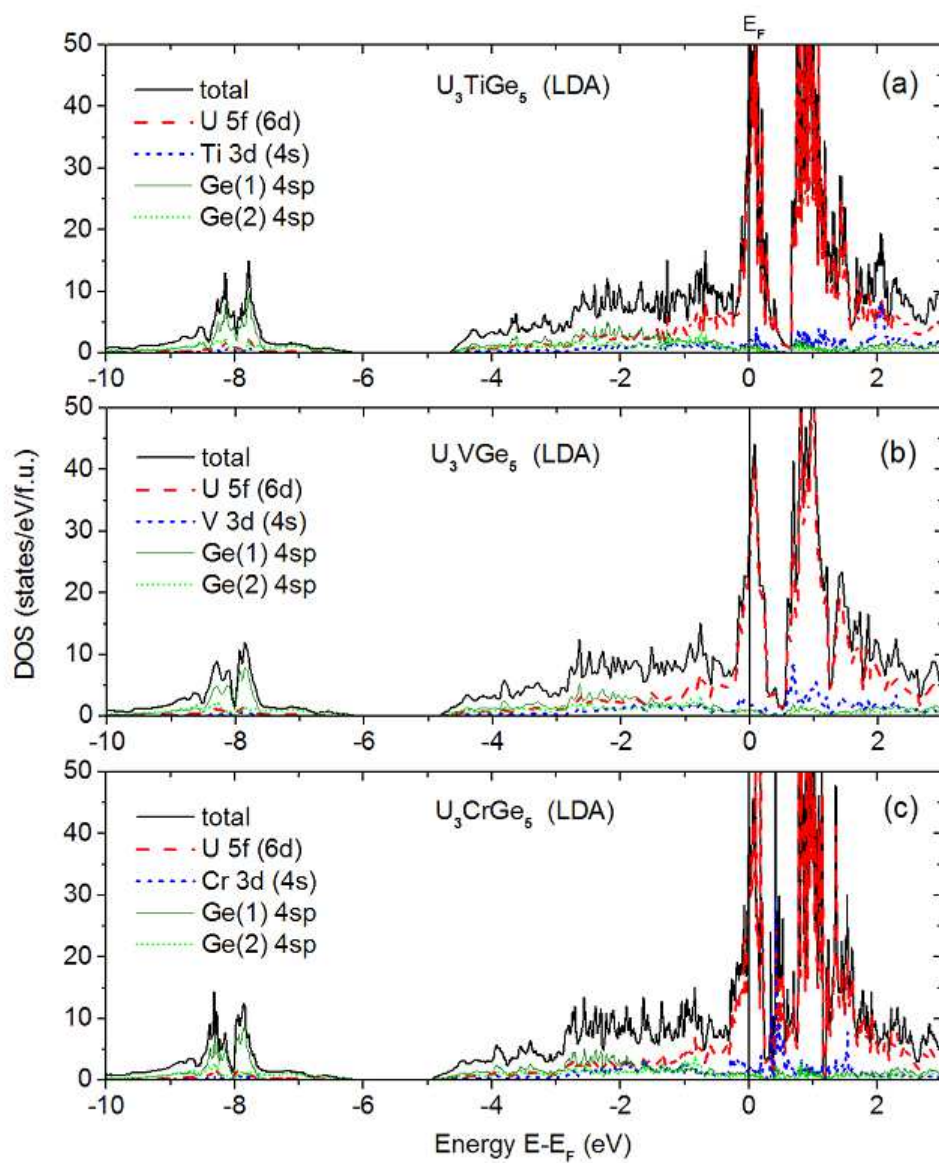
Fig. 7 Total and partial DOS's of U_3TGe_5 systems with T = \text{Ti} (a), \text{V} (b) and \text{Cr} (c) calculated for their non-magnetic states (LDA).
