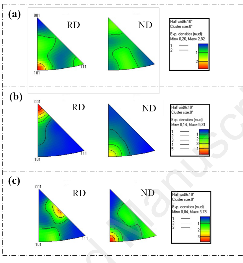
Fig. 4. Inverse pole figures of the solution treated alloy samples: ST-700-30 (a); ST-800-30 (b); ST-900-30 (c). RD is parallel to the tensile direction.
