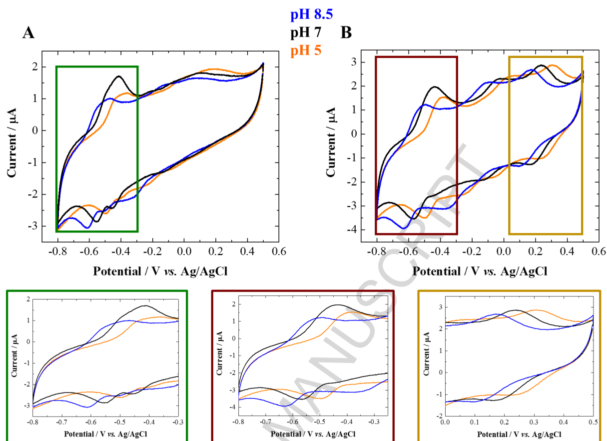
Figure 3. Top: Cyclic voltammograms recorded at 100 \text{ mV s}^{-1} on (A) \text{Fcc}_3 -modified and (B) catechol/ \text{Fcc}_3 -modified pyrolytic graphite electrodes in 0.1 \text{ M} phosphate buffer aqueous electrolyte successively recorded at pH 7 (black), pH 8.5 (blue) and pH 5 (orange) under inert atmosphere (Ar). Bottom: Focus on portions of figures A and B.
