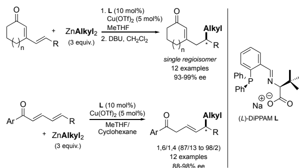
Scheme 1. Cu(OTf) 2 /DiPPAM L efficiently catalyzed 1,6-ACA of dialkylzinc reagents to cyclic and acyclic \alpha,\beta,\gamma,\delta -dienones.
