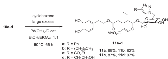
Scheme 5 Debenzylation in order to restore the catechol moiety and get the targeted triazoles 11a–d .
