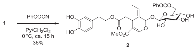
Scheme 1 Selective benzylation of oleuropein 1 .
