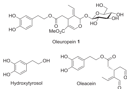
Fig. 1 Chemical structures of oleuropein 1 , hydroxytyrosol and oleacein.
