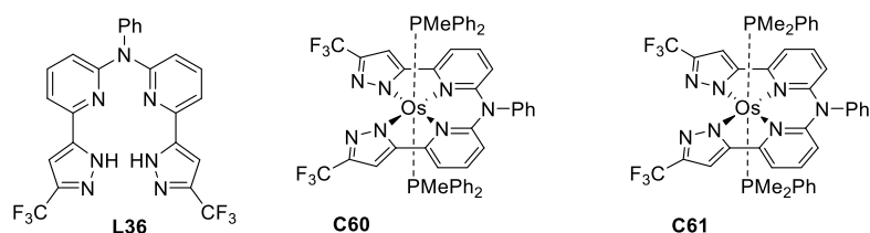
Figure 26 structure of ligand L36 and osmium(II) complexes [Os( L36 )(PMePh 2 ) 2 ] C60 and [Os( L36 )(PMe 2 Ph) 2 ] C61
