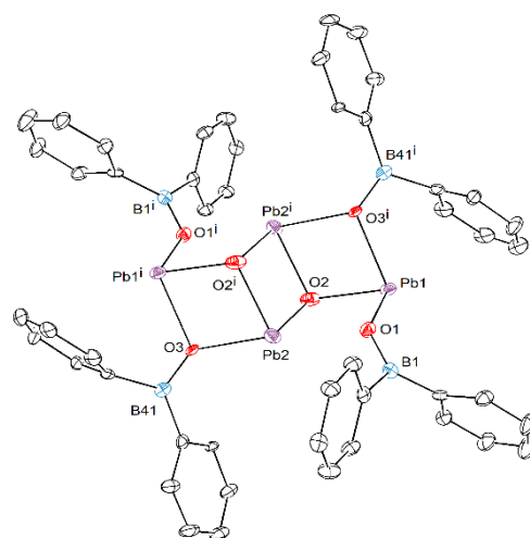
Figure 4. ORTEP representation of the molecular solid-state structure of [Pb_4(\mu_3-O)_2\{\mu_2-OB(2,4,6- i Pr_3-C_6H_2)_2\}_4] ( 4 ). Ellipsoids at the 50% probability level. H atoms and i Pr groups not represented for clarity. Representative bond lengths (Å) and angles ( ^\circ ): Pb1–O2 = 2.201(5), Pb1–O1 = 2.231(5), Pb1–O3 i = 2.350(5), Pb2–O2 = 2.206(5), Pb2–O2 i = 2.231(5), Pb2–O3 = 2.437(5); O2–Pb1–O1 = 81.08(18), O2–Pb1–O3 i = 76.85(17), O1–Pb1–O3 i = 100.50(17), O2–Pb2–O2 i = 77.70(2), O2–Pb2–O3 = 102.02(17), O2 i –Pb2–O3 = 74.52(17). Symmetry transformations used to generate equivalent atoms: -x, -y, -z .
