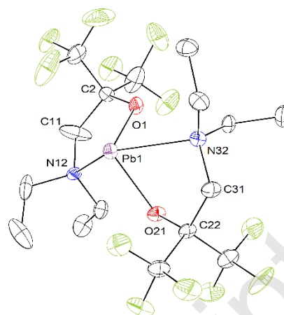
Figure 2. ORTEP representation of the molecular solid-state structure of [(RO^F)_2Pb] ( 2 ). Ellipsoids at the 50% probability level. H atoms omitted for clarity. Only one site occupancy for the disordered CF_3 group is depicted. Representative bond lengths (Å) and angles ( ^\circ ): Pb1-O1 = 2.185(3), Pb1-O21 = 2.214(3), Pb1-N32 = 2.572(4), Pb1-N12 = 2.608(4); O1-Pb1-O21 = 98.34(13), O1-Pb1-N32 = 83.81(12), O21-Pb1-N32 = 68.99(13), O1-Pb1-N12 = 69.90(13), O21-Pb1-N12 = 82.82(13), N32-Pb1-N12 = 138.08(13). Torsion angles ( ^\circ ): O1-C2-C11-N12 = 11.50(9), O21-C22-C31-N32 = -7.30(6)
