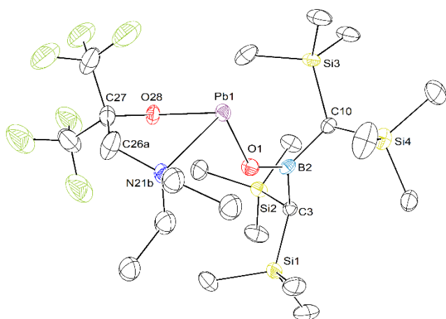
Figure 3. ORTEP representation of the molecular solid-state structure of [\{RO\}PbOB\{CH(SiMe_3)_2\}_2] ( 3 ). Ellipsoids at the 50% probability level. Only the main component (82% site occupancy) is depicted. H atoms omitted for clarity. Representative bond lengths (Å) and angles ( ^\circ ): Pb1–O1 = 2.128(2), Pb1–O28 = 2.181(4), Pb1–N21B = 2.448(4); O1–Pb1–O28 = 87.25(19), O1–Pb1–N21B = 94.65(12), O28–Pb1–N21B = 71.60(2), O1–B2–C3 = 118.20(3), O1–B2–C10 = 123.40(3), C3–B2–C10 = 118.40(3), B2–O1–Pb1 = 132.90(2). Torsion angle ( ^\circ ): N21B–C26A–C27–O28 = -9.50(6) .
