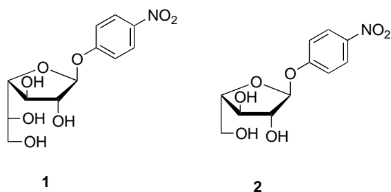
Fig. 1. Chemical structures of pNP β-D-Galf 1 and its analogue pNP α-L-Araf 2 .
