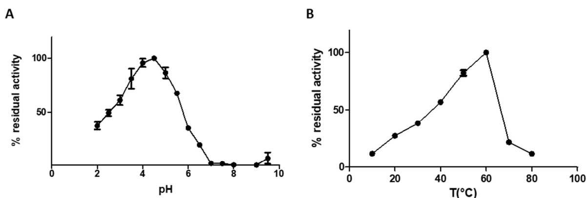
Fig. 4. A: Influence of pH on Gal f -ase hydrolytic activity towards p NP \beta -D-Gal f 1 . B: Influence of temperature on Gal f -ase hydrolytic activity towards p NP \beta -D-Gal f 1 . Error bars correspond to the SD of 3 independent measurements.
