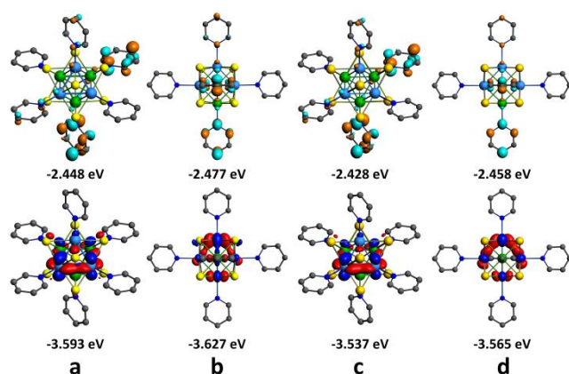
Figure 4. HOMO (bottom) and LUMO (top) orbitals of the different isomers of the [\text{Re}_3\text{Mo}_3\text{Q}_8(\text{py})_6] (Q = S, Se) clusters. a – fac - [\text{Re}_3\text{Mo}_3\text{S}_8(\text{py})_6] , b – -mer - [\text{Re}_3\text{Mo}_3\text{S}_8(\text{py})_6] , c – fac - [\text{Re}_3\text{Mo}_3\text{Se}_8(\text{py})_6] , d – mer - [\text{Re}_3\text{Mo}_3\text{Se}_8(\text{py})_6] .
