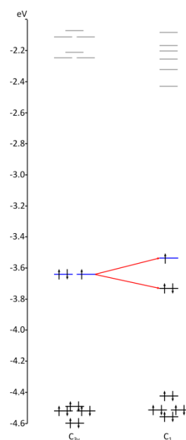
Figure 6. Energy levels diagram in near frontier orbital region for fac - isomer of the [Re 3 Mo 3 Se 8 (py) 6 ] cluster with C_{3v} (left) and C_1 (right) symmetries.
