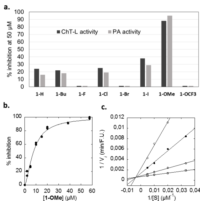
Figure 5. Effects of tryptanthrins on human 20S constitutive proteasome (pH 8, 37 °C). a. Inhibition of the ChT-L and PA activities by 50 \mu M tryptanthrins 1-R . b. Inhibition profile of the PA activity (substrate Z-LLE- \beta NA, 50 \mu M) by 1-OMe showing an IC 50 of 8.0 \pm 0.5 \mu M. c. Double-reciprocal Lineweaver-Burk plot for the inhibition of the ChT-L activity by tryptanthrin 1-OMe ; [20S proteasome] = 0.3 nM; [ 1-OMe ] = 0 \mu M ( \square ); [ 1-OMe ] = 10 \mu M ( \circ ); [ 1-OMe ] = 20 \mu M ( \bullet ); [ 1-OMe ] = 38 \mu M ( \diamond ); F.U., fluorescence arbitrary unit; S, substrate Suc-LLVY-AMC.
