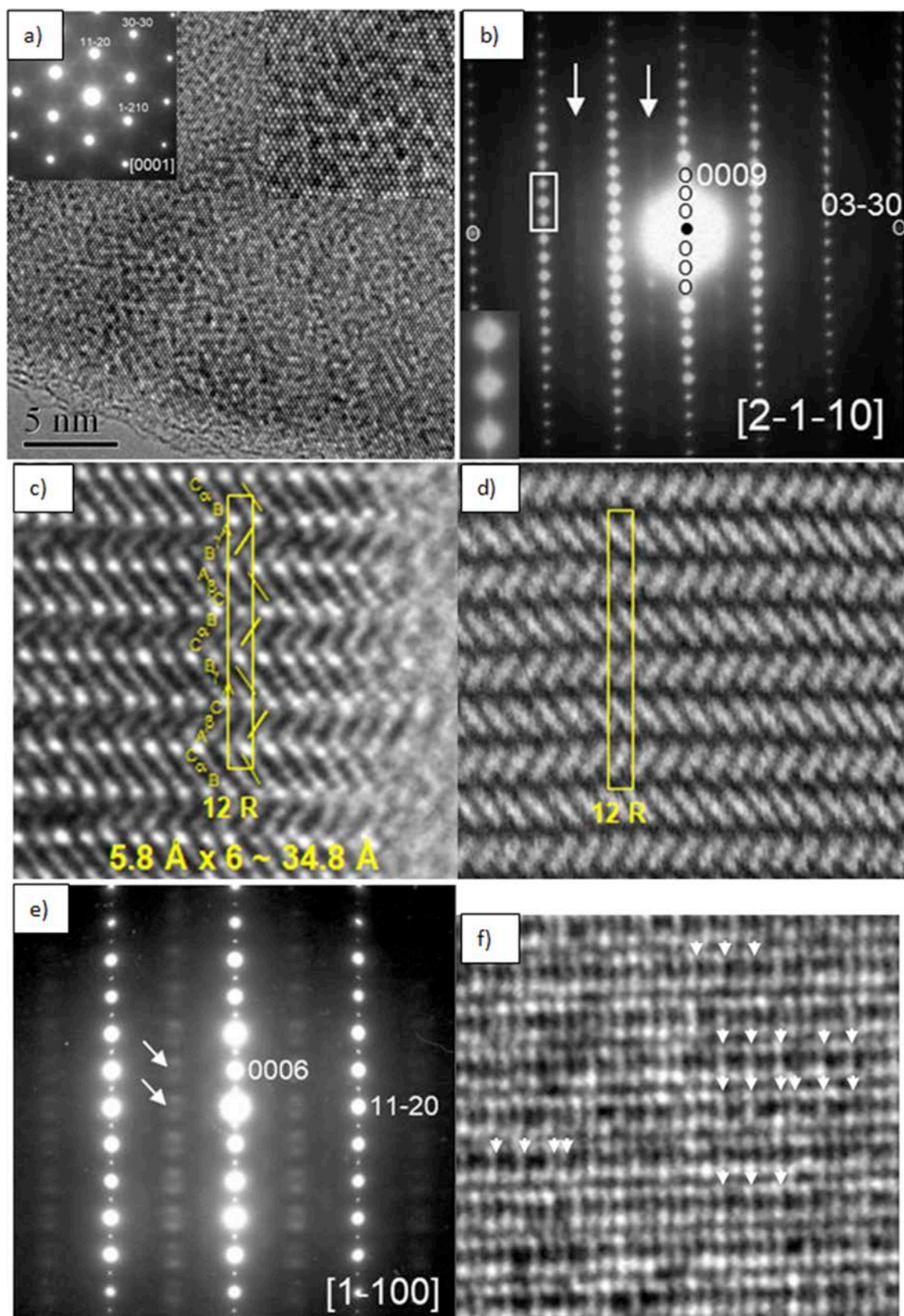
Fig. 8. (a) HRTEM image of 12R-M 1+x S 2 (with x ~ 0.21, M = Ge/Ti) taken along the [0001] zone axis; the insets show the corresponding SAED pattern and an enlargement of the micrograph, (b) [2-1-10] zone axis SAED pattern, the inset shows streaking running along c^*
