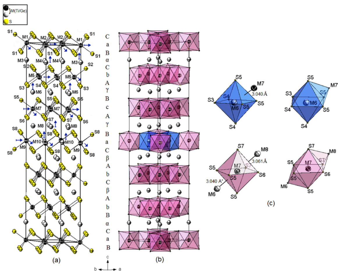
Fig. 3. Crystal structure of 12R-super M_{1.206}S_{1.91} ( M = \text{Ge/Ti} ). (a) Prism-prism-octahedron-octahedron packing of sulphur layers. (b) Clinographic view of the edge sharing MS_6 octahedrons. (c) Distorted bicapped and monocapped octahedral coordination around metal atoms showing the short M-M distances. The colour key is as in Fig. 1.
