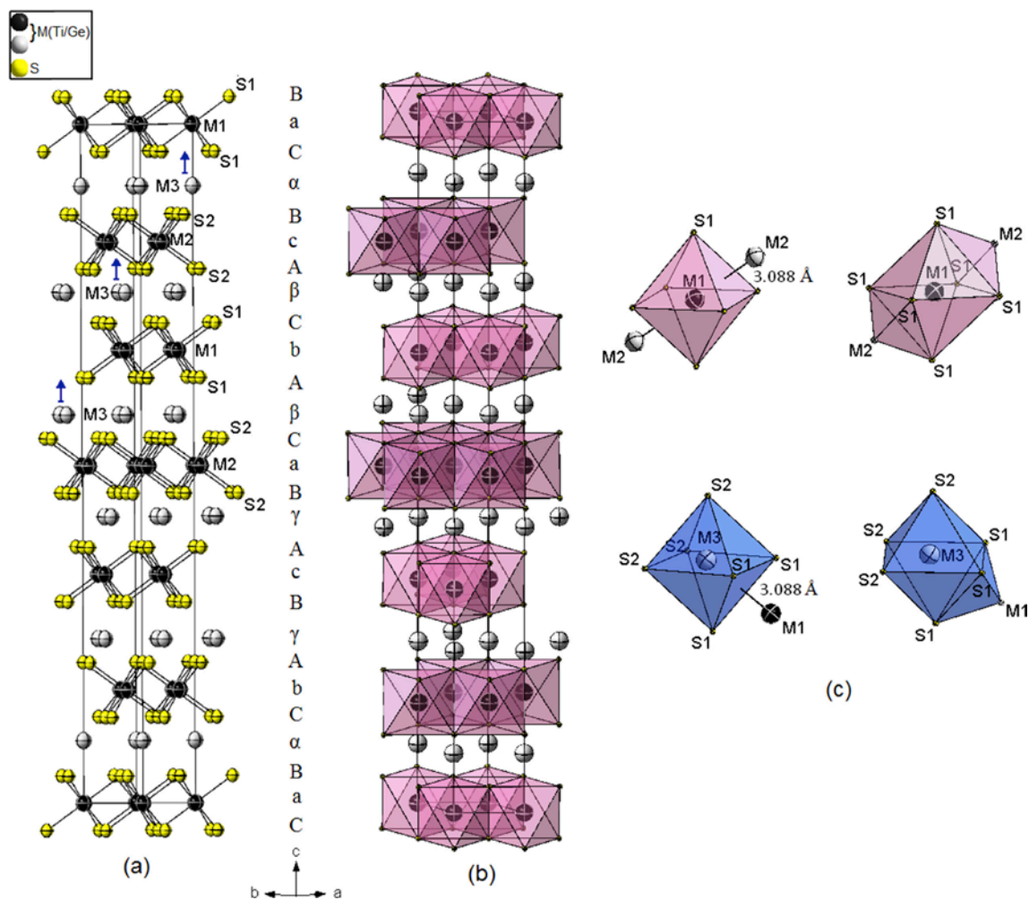
Fig. 2. Crystal structure of 12R\text{-}M_{1.111}\text{S}_2 ( M = \text{Ge/Ti} ). (a) Prism -prism-octahedron-octahedronpacking of sulphur layers. (b) Clinographic view of the edge sharing \text{MS}_6 octahedrons. (c) Distorted bicapped and monocapped octahedral coordination around metal atoms showing the short M-M distances. The colour key is as in Fig. 1.
