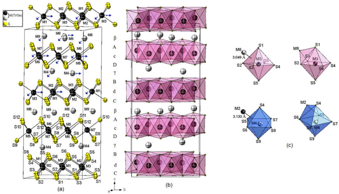
Fig. 4. Crystal structure of (4H)_2-M_{1.244}S_{1.945} (M = Ge/Ti) superstructure. (a) Prism - octahedron- prism –octahedron packing of sulphur layers. (b) Clinographic view of the edge sharing MS_6 octahedrons. (c) Distorted monocapped octahedral coordination around metal atoms showing the short M-M distances. The colour key is as in Fig. 1.
