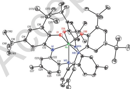
Fig. 46 50% thermal ellipsoid plot of the seven-coordinate Mo(VI) complex [Mo(MeClamp)].3C 6 H 6 ( 103 ). Hydrogen atoms are omitted for clarity. Reproduced with permission [322]. Copyright 2015 The Royal Society of Chemistry.
