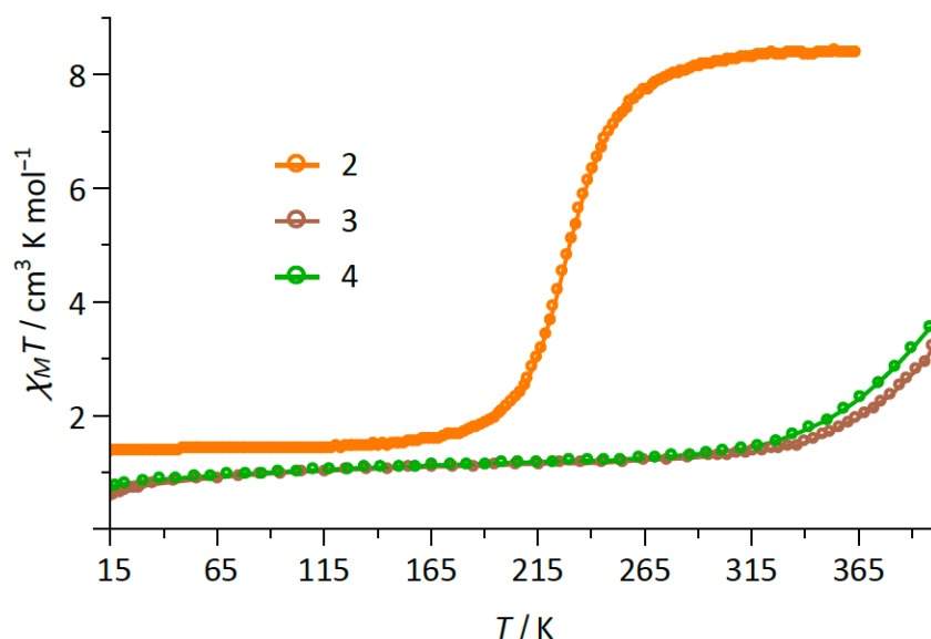
Fig. 2. Magnetic properties of 2-4 depicted as the \chi_{MT} versus T curve.
