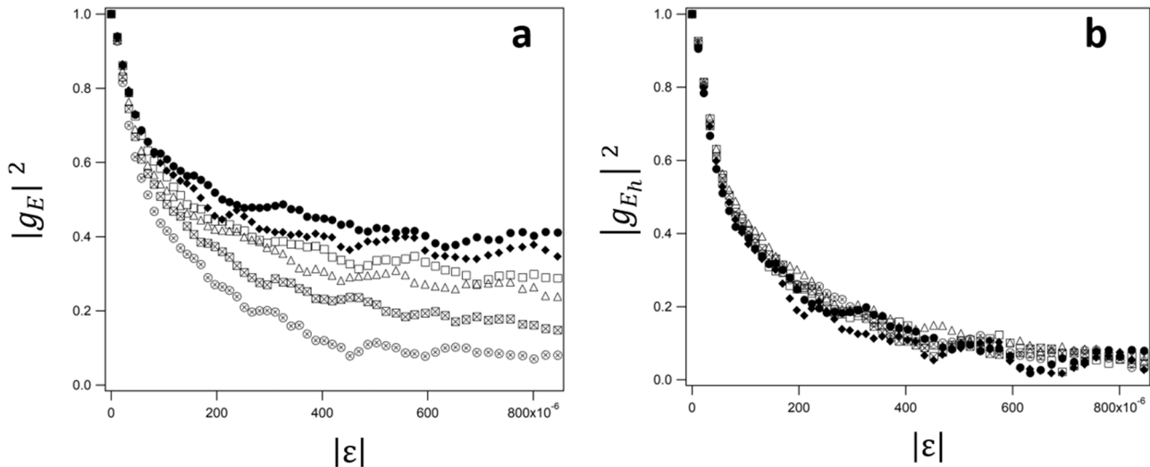
Fig. 4. (a) Correlation functions |g_E|^2 vs. |\epsilon| for six different metapixels of size 96 \times 96 px. (b) Correlation function for homogeneous illumination as computed from (11).
