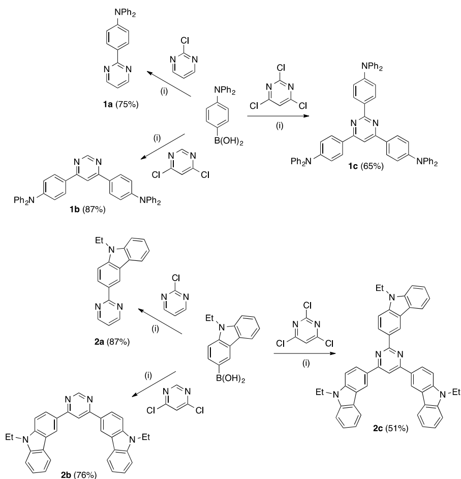
Scheme 1. Preparation of pyrimidines 1 and 2 . (i) Toluene, Pd(PPh 3 ) 4 , Na 2 CO 3 aq., EtOH, Δ, 15 h.
