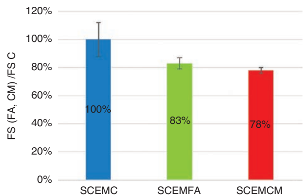
FIGURE 9. Evolution of the fraction of flexural strengths of SCEMs based on mineral additions compared to control SCEM.
