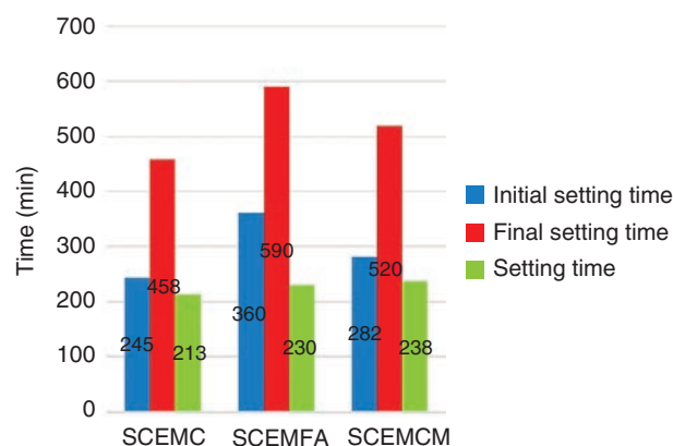
FIGURE 5. The initial times of setting, the final of setting and the setting time of SCCEMs studied.
