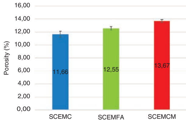
FIGURE 12. Porosity accessible to water of the different SCEMs studied.
