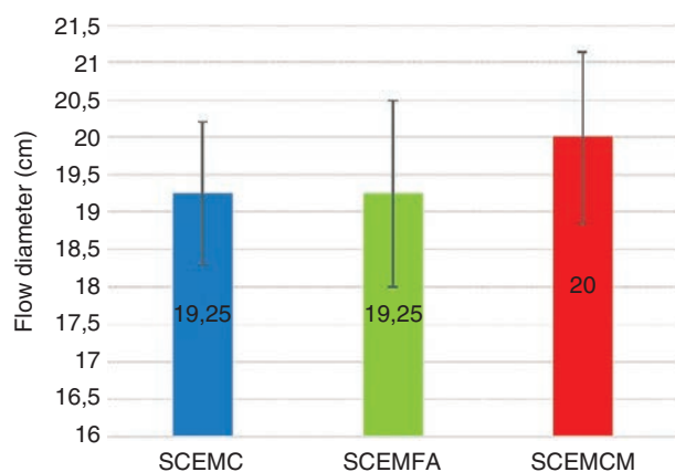
FIGURE 4. Slump flow variation of SCCEMs studied.
