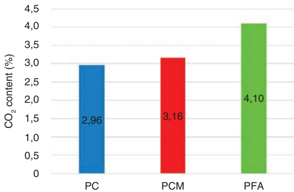
FIGURE 11. CO 2 content of the mortar pastes studied.
