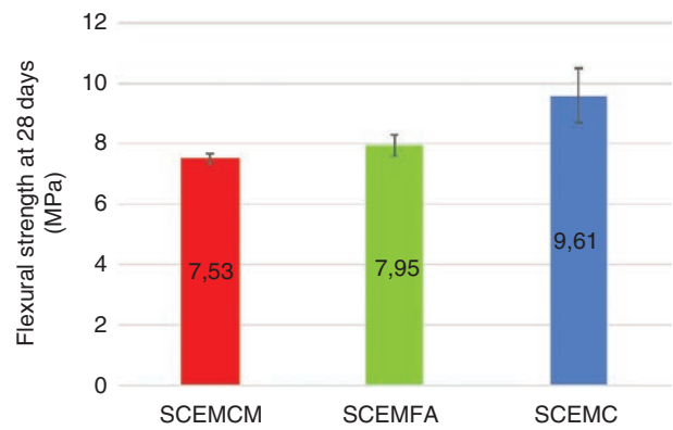
FIGURE 8. Evolution of flexural strengths of SCEMs, at 28 days
