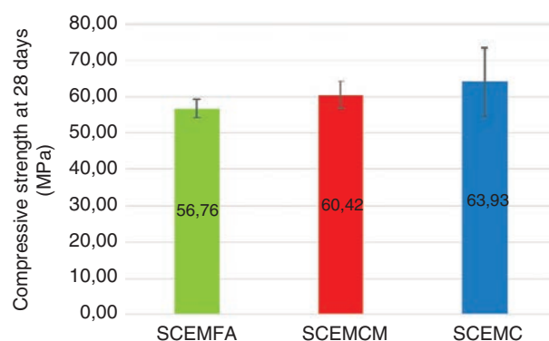
FIGURE 6. Evolution of the compressive strength at 28 days of SCCEMs studied.
