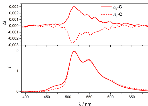
Figure 5. Emission and CPL spectra of \Delta I_{\text{r}}(-)\text{-C} (solid red) and \Delta I_{\text{r}}(+)\text{-C} (dashed red) in carefully deaerated \text{CH}_2\text{Cl}_2 solutions at rt ( C \sim 1.10^{-5} M). Excitation wavelength \lambda_{\text{ex}} at 350nm.
