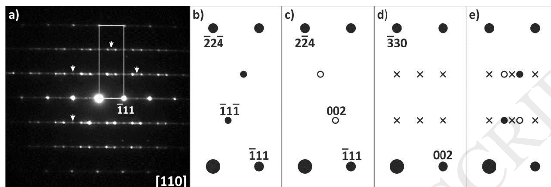
Fig. 8. (a) SAED pattern of a grain of the sulfurized powder along the [110] zone axis. The main reflections are attributed to the sphalerite crystalline structure with twinning and the arrows show some weak reflections of the wurtzite 2H crystalline structure. Simulations of reflection positions are drawn on (b) first twin of sphalerite, (c) second twin of sphalerite, (d) wurtzite and (e) superposition of all domains
