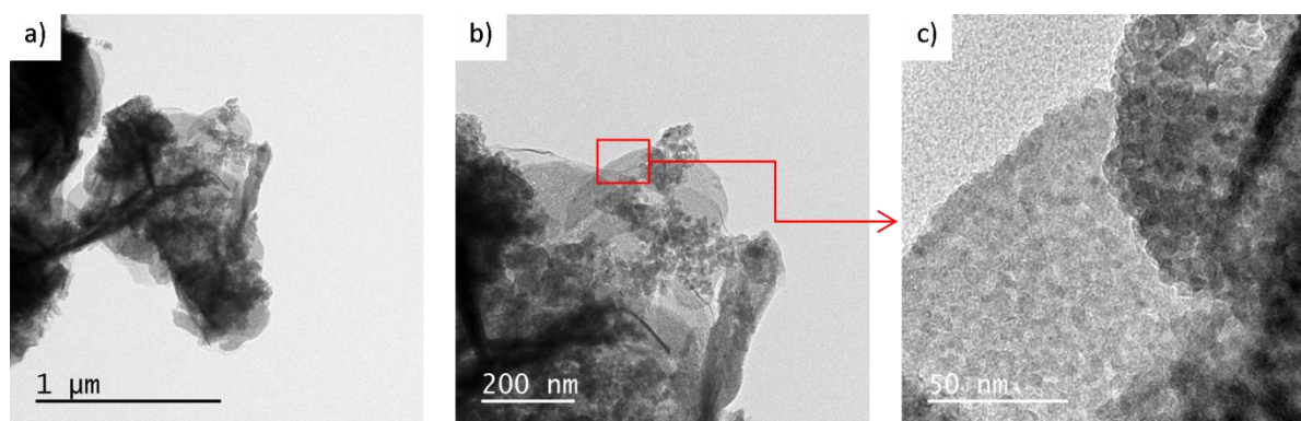
Fig. 5. Brightfield TEM micrographs of the ZnS raw powder
