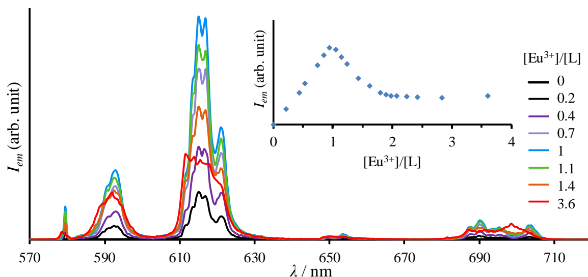
Figure 3. Evolution of the luminescence spectra of a solution of L upon titration by \text{EuCl}_3 (0.01 M TRIS/HCl, pH = 7.1, \lambda_{exc} = 267 \text{ nm} ). Inset: Evolution of the emission intensity at 616 nm as a function of the [\text{Eu}^{3+}]/[\text{L}] ratio. [\text{L}] = 5.0 \times 10^{-5} \text{ M} .
