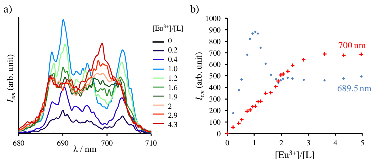
Figure 4. a) Enlargement of the variations on the ^5D_0 \rightarrow ^7F_4 transition of a solution of L upon titration by \text{EuCl}_3 (0.01 M TRIS/HCl, pH = 7.1, \lambda_{exc} = 267 nm). b) Evolution of the emission intensity at 689.5 nm and 700 nm as a function of the [\text{Eu}^{3+}]/[\text{L}] ratio.
