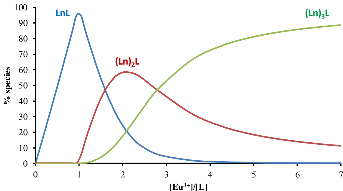
Figure 5. Theoretical representation of the species formed upon addition of \text{LnCl}_3 ( \text{Ln} = \text{Eu}, \text{Tb} ) in an aqueous solution of ligand L ( [\text{L}] = 5.00 \times 10^{-5} \text{ M} , \text{TRIS}/\text{HCl} 0.01\text{M} , \text{pH} = 7.1 , calculated with \text{Log } \beta_{\text{LnL}} = 15.7 , \text{Log } \beta_{(\text{Ln})_2\text{L}} = 21.1 and \text{Log } \beta_{(\text{Ln})_3\text{L}} = 25.5 ).
