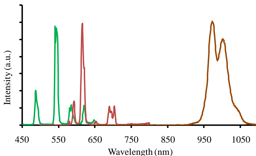
Figure 9. Luminescence spectra of [TbL], [EuL] and [YbL] in water upon ligand excitation (normalized to their maximum of emission, \lambda_{\text{exc}} = 269 nm, H 2 O, TRIS/HCl 0.01 M, pH 7.0).
