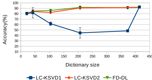
Figure 4: Accuracy of classification of the LC-KSVD and FD-DL algorithms varying the number of dictionary atoms.
