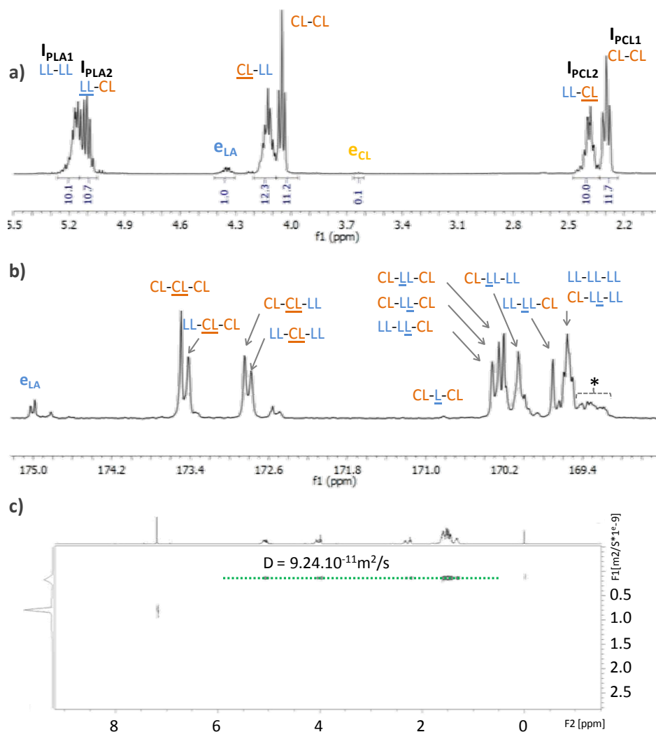
Figure 4. (a) ^1\text{H} (400.2 MHz, r.t.) and (b) ^{13}\text{C} (100.6 MHz, r.t.) NMR spectra of a P(LA-co-CL) copolymer in \text{CDCl}_3 (Table 1, run 3); LL and L refer to lactidyl and lactoyl units, respectively; * epimerized LL-LL-LL sequences; (c) DOSY NMR spectrum ( \text{CDCl}_3 , 400.2 MHz, r.t.) of pure copolymer (Table 1, run 3).
