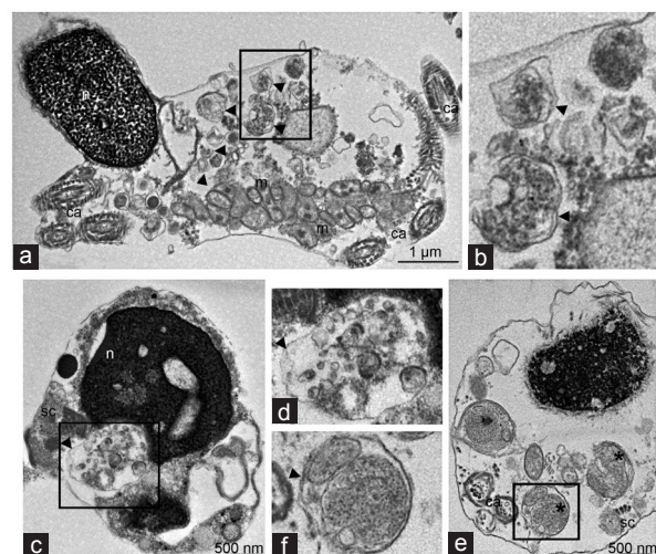
Figure 4: Transmission electron microscopy analysis of cryptorchid spermatozoa reveals autophagic vacuoles. (a) Longitudinal section of cryptorchid spermatozoon, exhibiting the nucleus with uncondensed chromatin, partly detached nuclear envelope (arrow), and coiled axoneme (ca). The large cytoplasmic droplet contains the autophagic vacuoles (arrowheads), located next to irregular gyres of damaged mitochondria (m). (b) A higher magnification of the selected area from a. Note double membrane-limited autophagic vesicles (arrowheads) containing partly degraded vesicular material. Cross-sections of cryptorchid spermatozoa pass through the postequatorial segment of the heads, which manifest (c) chromatin rarefaction and (e) granulation. (e) Coiled aberrant axonemes (ca) and the fragments of segmented columns (sc) forming conico-cylindrical sleeve are scattered in the cytoplasm. (d) Double-membrane-limited autophagosomes (arrowheads) filled with vesicular material locate in close proximity to (c) the nucleus, (e) while partly degraded mitochondria (asterisk) are next to plasma membrane and seemingly fusion with it. d and f are higher magnifications from selected area from c and e, respectively showing (d) double membrane-limited autophagosomes (arrowhead) enclosing vesicles or (f) mitochondria. m: mitochondria; n: nucleus.
