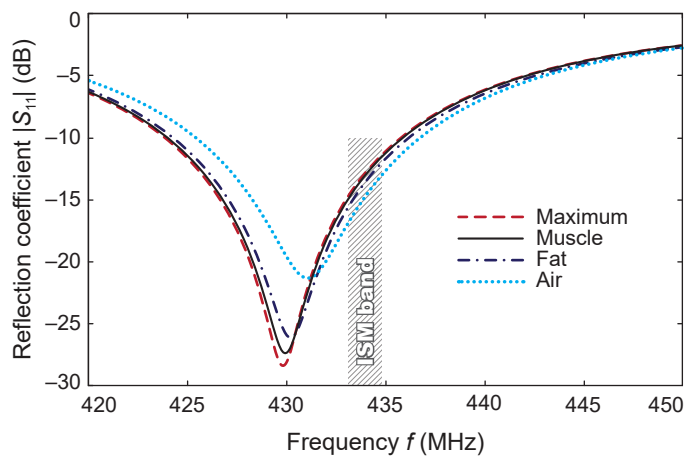
Fig. 3. Reflection coefficient |S_{11}| of the proposed antenna computed in air and in a \varnothing 100\text{-mm} spherical phantom with various EM properties.
