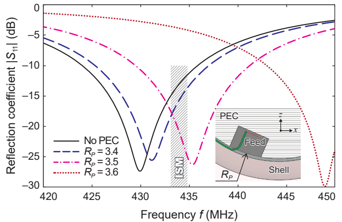
Fig. 6. Effect of capsule inner components on the antenna performance: computed reflection coefficients |S_{11}| for various radii of a PEC cylinder spanning the full length of the antenna. The inset shows the PEC cylinder ( R_P = 3.6 mm) with a pocket to accommodate the waveguide port.
