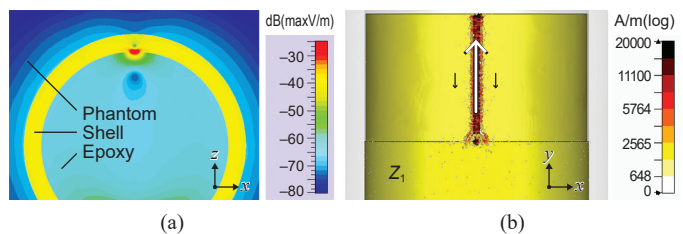
Fig. 4. Fields of the antenna at 434 \text{ MHz} . (a) |\mathbf{E}| -field ( \text{dBmax} ) distribution on the x - z plane orthogonal to Z_2 section ( 2 \text{ mm} from Z_1 - Z_2 transition). (b) Surface current distribution \log(I) ( \text{A}\cdot\text{m}^{-1} ) for the phase \varphi = 90^\circ .
