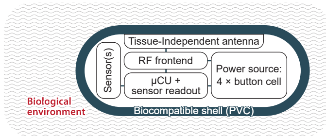
Fig. 1. Outline of the wireless pill-shaped device for biotelemetry. Tissue-independent antenna design ensures the detuning immunity.
