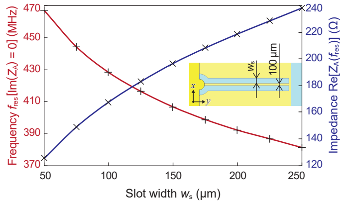
Fig. 5. Adjusting the operating band of the proposed antenna: effect of the coplanar slot width w_s on antenna complex impedance Z_A (inset shows the geometry of the coplanar segment Z_2 , w_s = 200 \mu\text{m} ).
