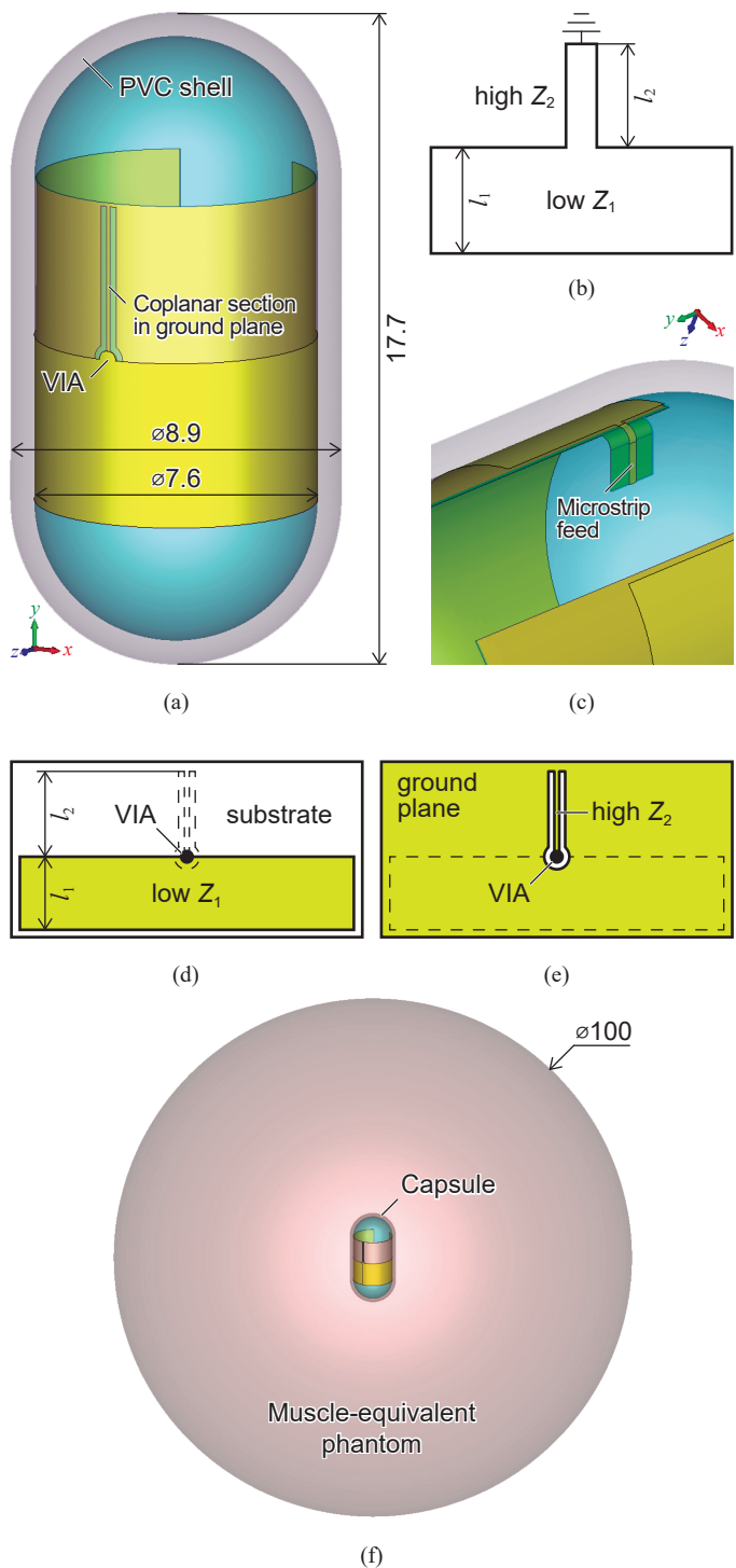
Fig. 2. Geometry and building blocks of the proposed capsule antenna (mm). (a) The antenna conforming to the inner surface of a 0.65-mm-thick PVC shell. (b) Theoretical representation: a quarter-wave stepped-impedance resonator. (c) Foldable microstrip feed connecting the antenna to the PCB (not shown). (d), (e) Top and bottom views, respectively, of the planar geometry of the antenna ( l_1 = 4.5 , l_2 = 4.2 ). (f) Simulation setup in CST MWS.
