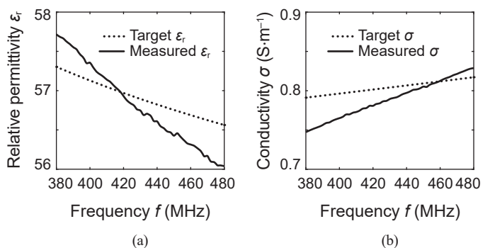
Fig. 8. Measured and target EM properties (at 25 \pm 0.5 \text{ }^\circ\text{C} ) of the muscle-equivalent liquid phantom used for the antenna measurements. (a) Relative permittivity \epsilon_r . (b) Conductivity \sigma .
