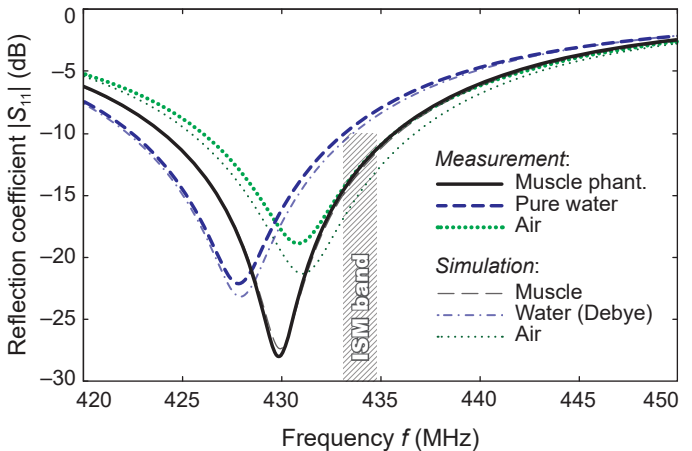
Fig. 9. Measured and computed reflection coefficients |S_{11}| of the proposed antenna in three media.
