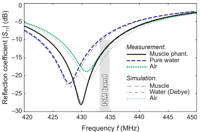
Fig. 9. Measured and computed reflection coefficients |S_{11}| of the proposed antenna in three media.
