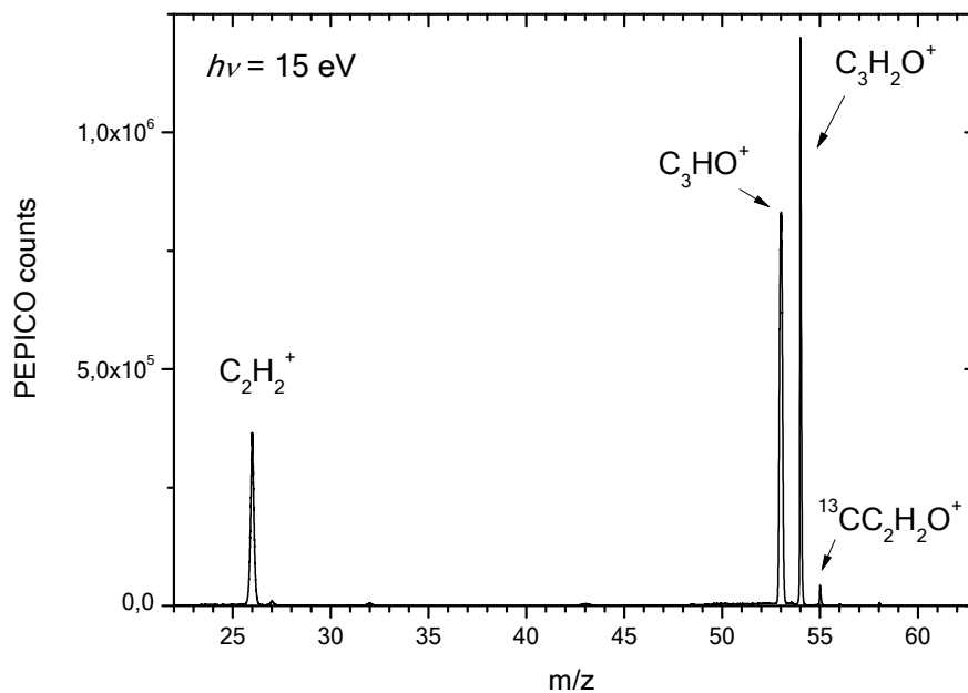
Figure 1: Time-of-flight mass spectrum of propynal photoionized at h\nu = 15 \text{ eV} .
