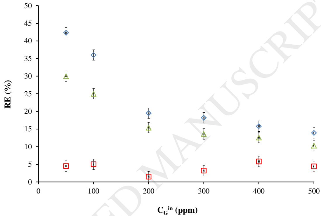
Figure 5: Removal efficiency vs H 2 S concentration at the inlet of filters in wet conditions at EBRT = 56 s (blue diamond: cellular concrete waste; green triangle: mixture of cellular concrete waste and expanded schist; red square: expanded schist).
