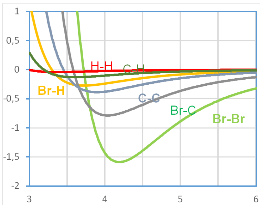
Figure 7- Variation of the atom-atom interaction forces as a function of the interatomic distance
