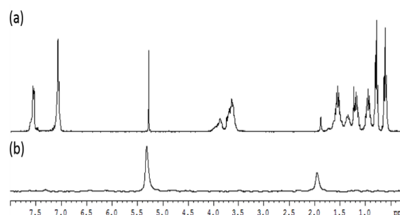
Figure 2. (a) ^1\text{H} NMR spectrum of compound 1 H in \text{CD}_2\text{Cl}_2 and (b) ^2\text{H} NMR spectrum of compound 1 D in \text{CH}_2\text{Cl}_2 solvent.
