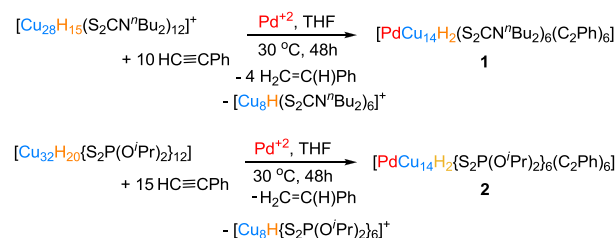
Scheme 1. Synthesis of compounds 1 and 2 .
