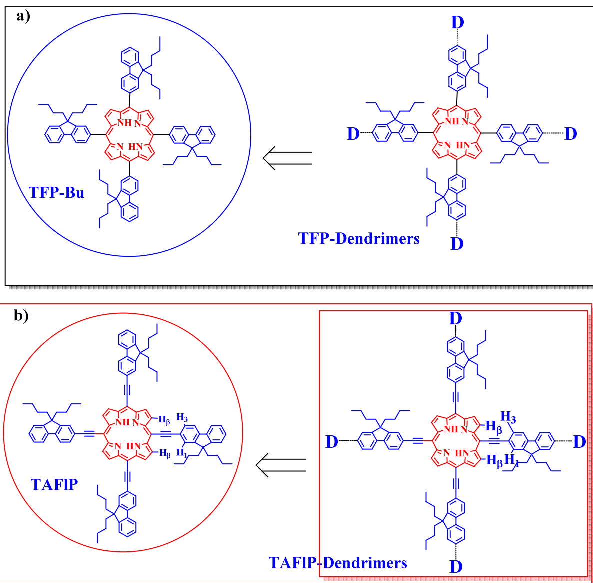
Fig. 4. a) Structure of reference compound TFP-Bu and corresponding TFP based dendrimers; b) target compound: new meso -alkynyl fluorenyl porphyrin TAFIP allowing the design of new TAFIP -based dendrimers
