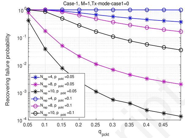
Fig. 14: Effect of N_{rep} parameter variation in Case-1 based FDP versus loss patterns (p_{pckt}, q_{pckt}) with M = 1 .
