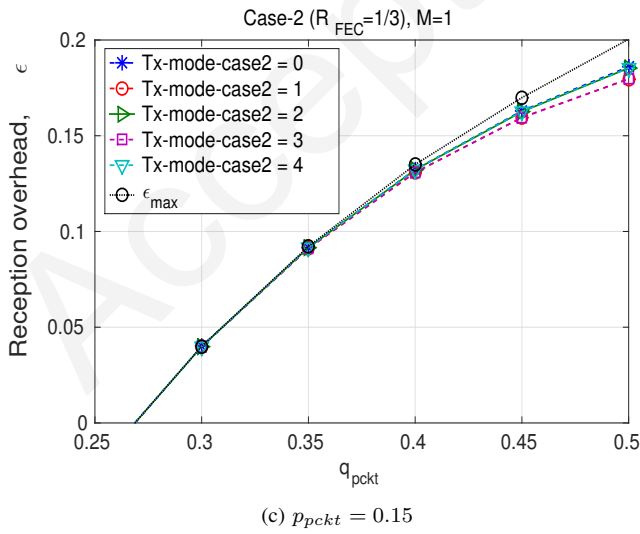
Fig. 19: Tx-mode-case2 parameter effect on reception overhead under different loss patterns ( p_{pkt} , q_{pkt} ) in Case-2.
