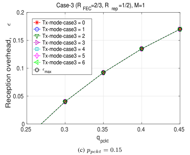
Fig. 20: Tx-mode-case3 parameter effect on reception overhead under different loss patterns ( p_{pkt} , q_{pkt} ) in Case-3.
