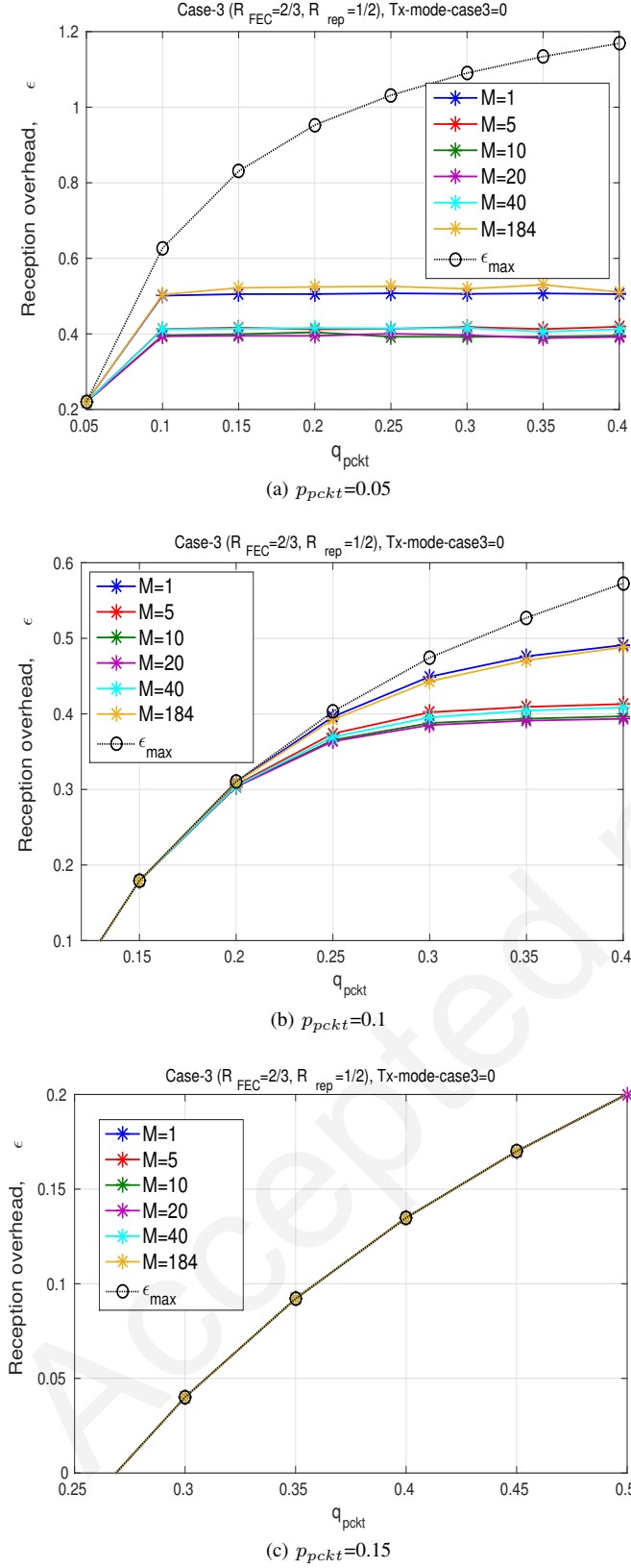
Fig. 17: Effect of parameter M on the reception overhead in Case-3 based FDP versus loss patterns (p_{pkt}, q_{pkt}) with R_{FEC} = \frac{2}{3} and R_{rep} = \frac{1}{2} .
