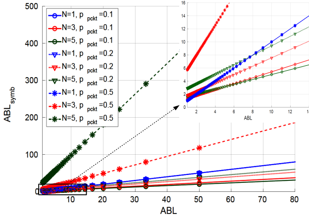
Fig. 10: ABL_{symp} versus ABL for different values of N and M = 1 . p_{pkt} = \frac{1}{AILD}
