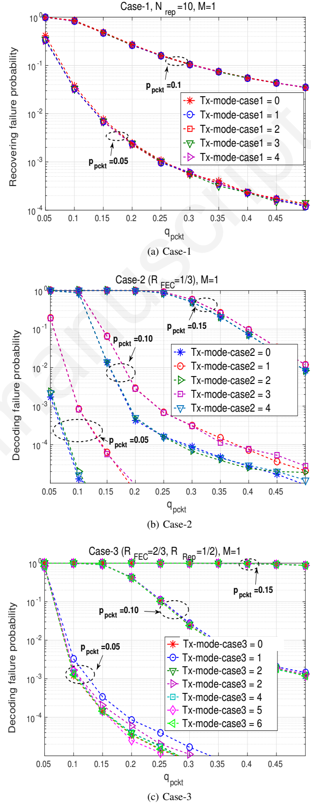
Fig. 18: Effect of the Tx-mode-case parameter variation on the recovering/decoding failure probability versus packet loss patterns (p_{pkt}, q_{pkt})
