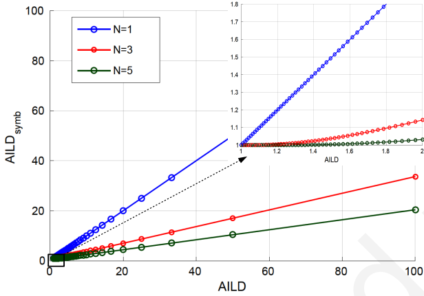
Fig. 11: AILD_{symp} versus AILD for different values of N and M = 1 .
