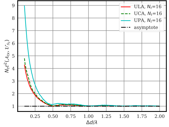
Fig. 2. Numerical evaluation of \mathcal{E}^2(\mathcal{A}_{tx}, \mathcal{U}_{S_2}) for various array types and increasing antenna spacing \Delta d . The values are normalized so the asymptote is 1.
