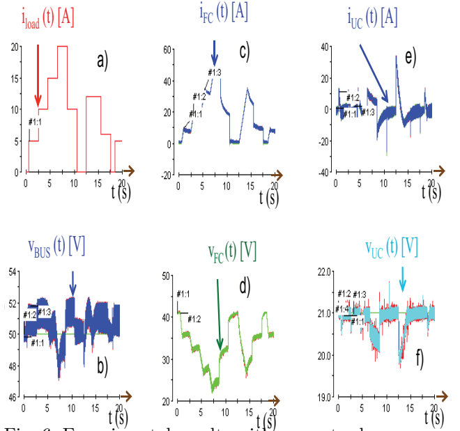
Fig. 6. Experimental results with converter losses.
