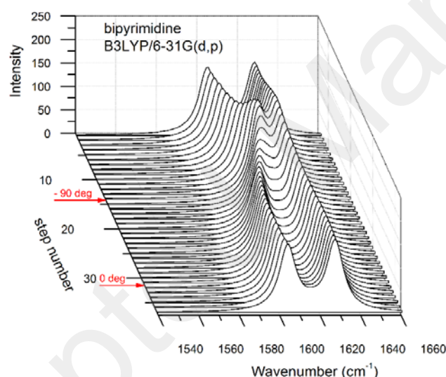
Figure 4. Vibrational band of the molecular core related to CN and CC stretching as a function of dihedral angle.
