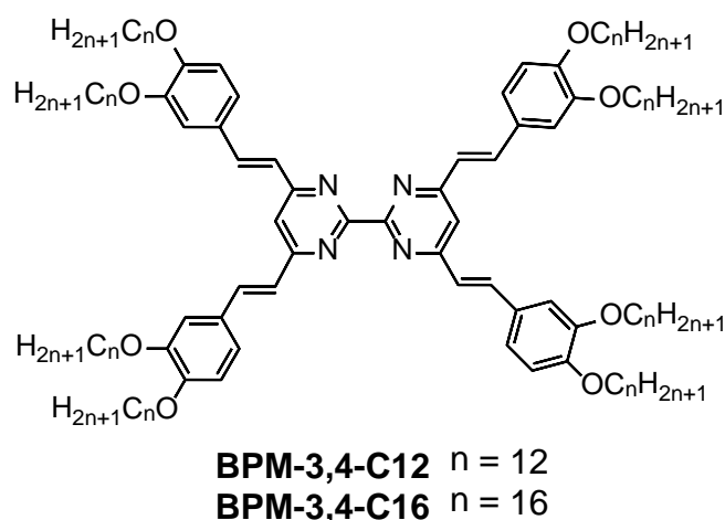
Scheme 1. Molecular structure of the chiral BPM compounds.
