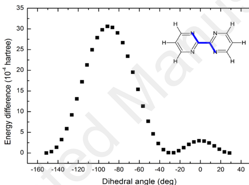
Figure 2. Total energy as a function of dihedral angle (the dihedral angle equals to 0° for the flat molecule).
