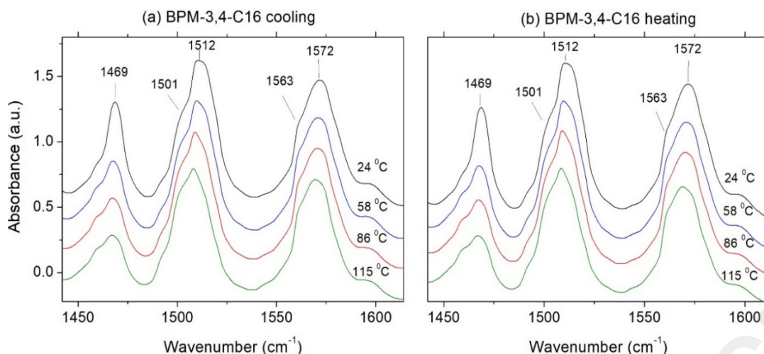
Figure 11. Temperature dependence of the IR absorption spectra of BPM-3,4-C16 thin films on cooling (a) and heating (b). Note that for clarity the spectra are separated along the absorbance axis.
