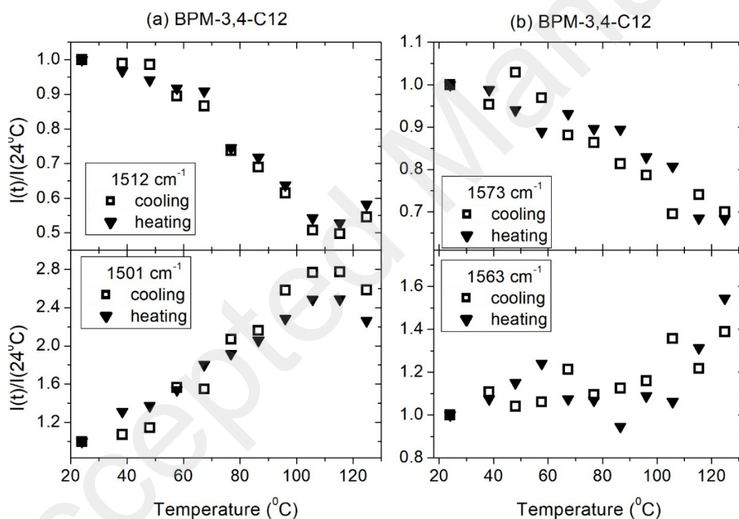
Figure 14. Temperature dependence of the integral intensity of the spectral features for thin layer of BPM-3,4-C12 on cooling and heating: (a) side-band at 1501 cm -1 and main band at 1512 cm -1 and (b) side-band at 1563 cm -1 and main band at 1573 cm -1 .
