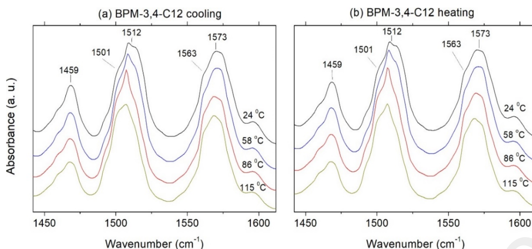
Figure 13. Temperature dependence of the IR absorption spectra of thin films of BPM-3,4-C12 on cooling (a) and heating (b). Note that for clarity the spectra are separated along the absorbance axis.
