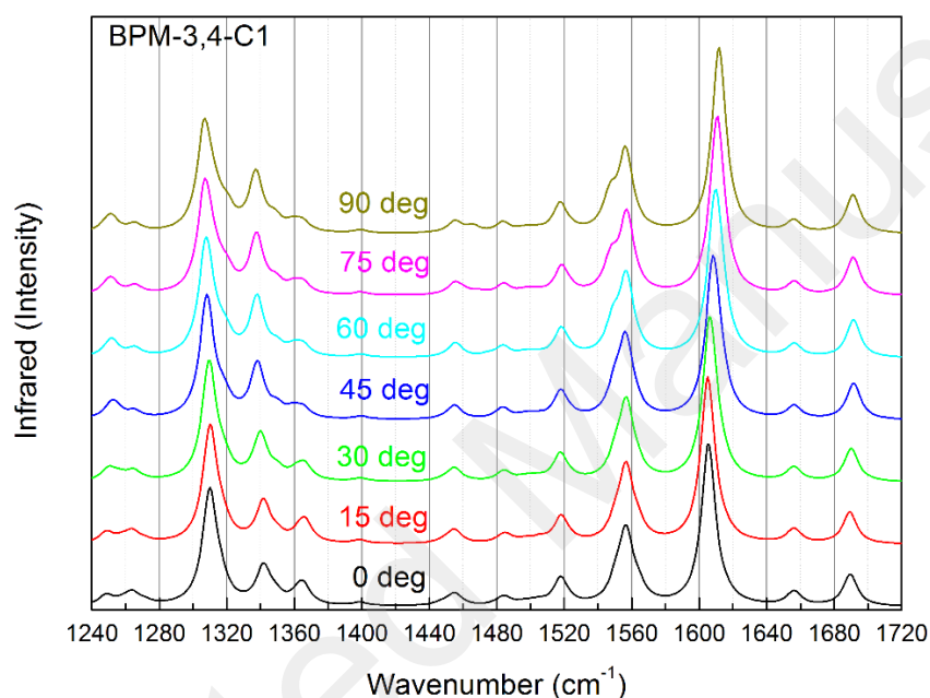
Figure 6. The simulated IR spectra of BPM-3,4-C1
