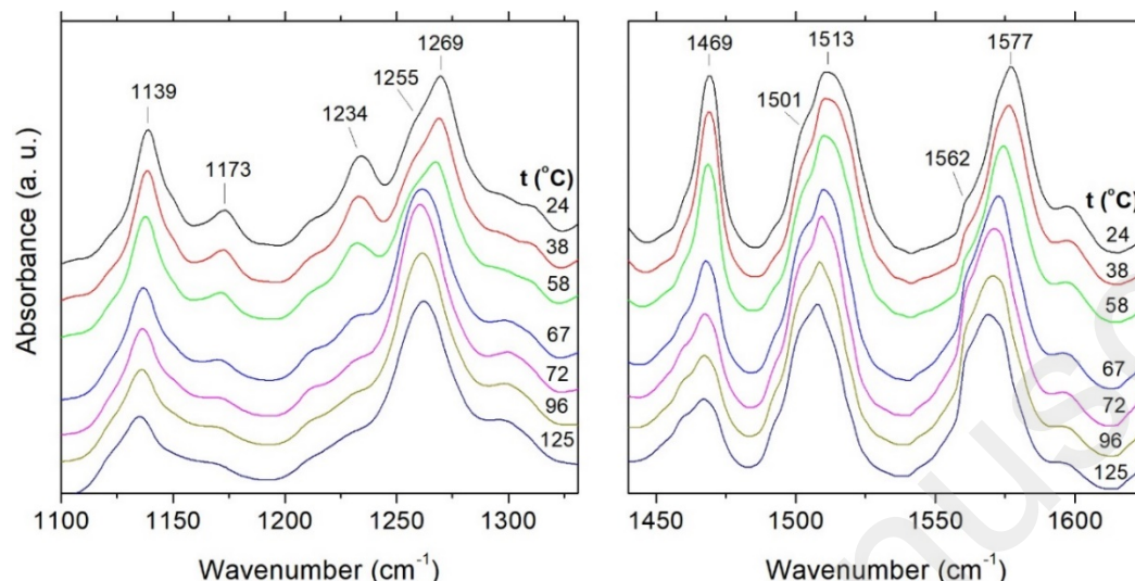
Figure 8. Temperature dependence of the IR absorption spectra of BPM-3,4-C16. Note that for clarity the spectra are separated along the absorbance axis.
