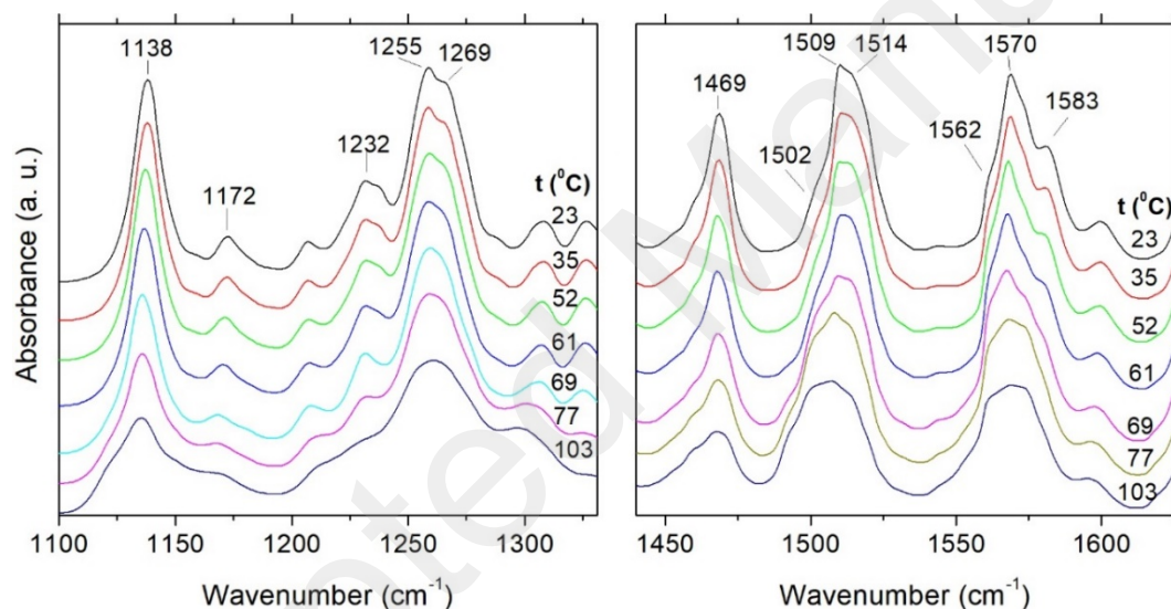
Figure 10. Temperature dependence of the IR absorption spectra of BPM-3,4-C12. Note that for clarity the spectra are separated along the absorbance axis.
