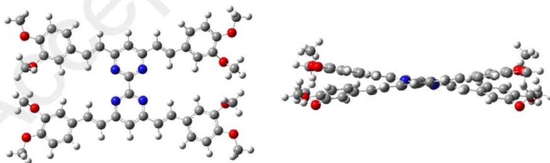
Figure 5. The equilibrium geometry of BPM-3,4-C1 molecule with dihedral angle frozen at 15^\circ .
