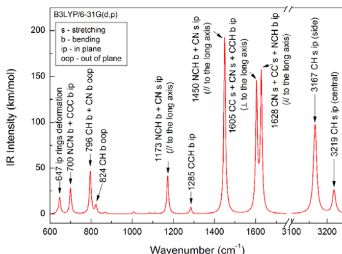
Figure 3. Calculated IR spectra of the molecular core.
