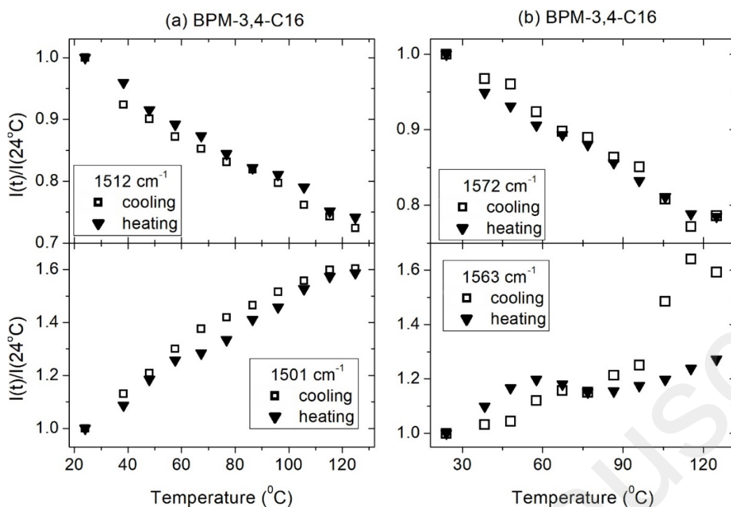
Figure 12. Temperature dependence of the integral intensities of spectral bands for thin layer of BPM-3,4-C16 on cooling and heating: (a) side-band at 1501 cm -1 and main-band at 1512 cm -1 and (b) side-band at 1563 cm -1 and main-band at 1572 cm -1 .
