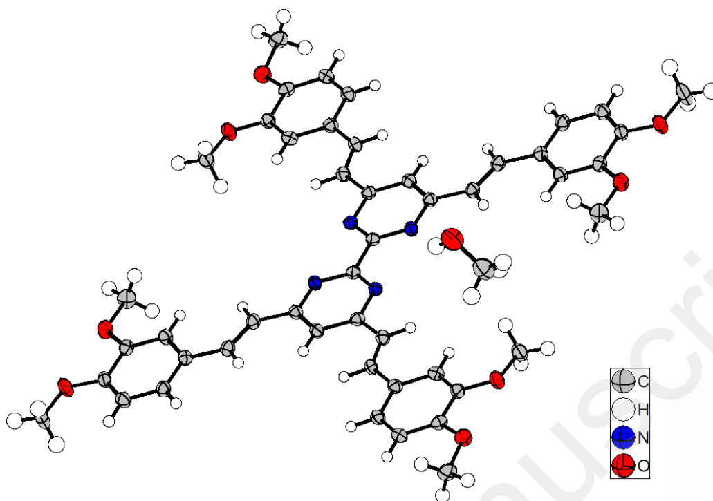
Figure 1. ORTEP view of BPM-3,4-C1 compound crystallized in presence of methanol molecules ( n = 1 ) (monoclinic, P 2_1/a , a = 17.3673(7) Å, b = 7.4860(4) Å, c = 17.5622(7) Å, \beta = 99.972(2)^\circ , Z = 2 ) (CCDC 1585239).
