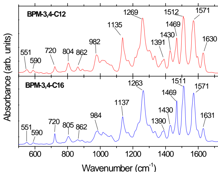
Figure 7. Room temperature infrared spectra of thin films of BPM-3,4-C12 and BPM-3,4-C16.
