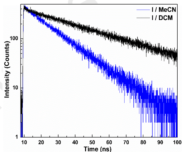
Fig. 9 Single exponential emission decays for I in aerated MeCN and DCM solutions ( \lambda_{em} = 645 nm and \lambda_{ex} = 405 nm).
