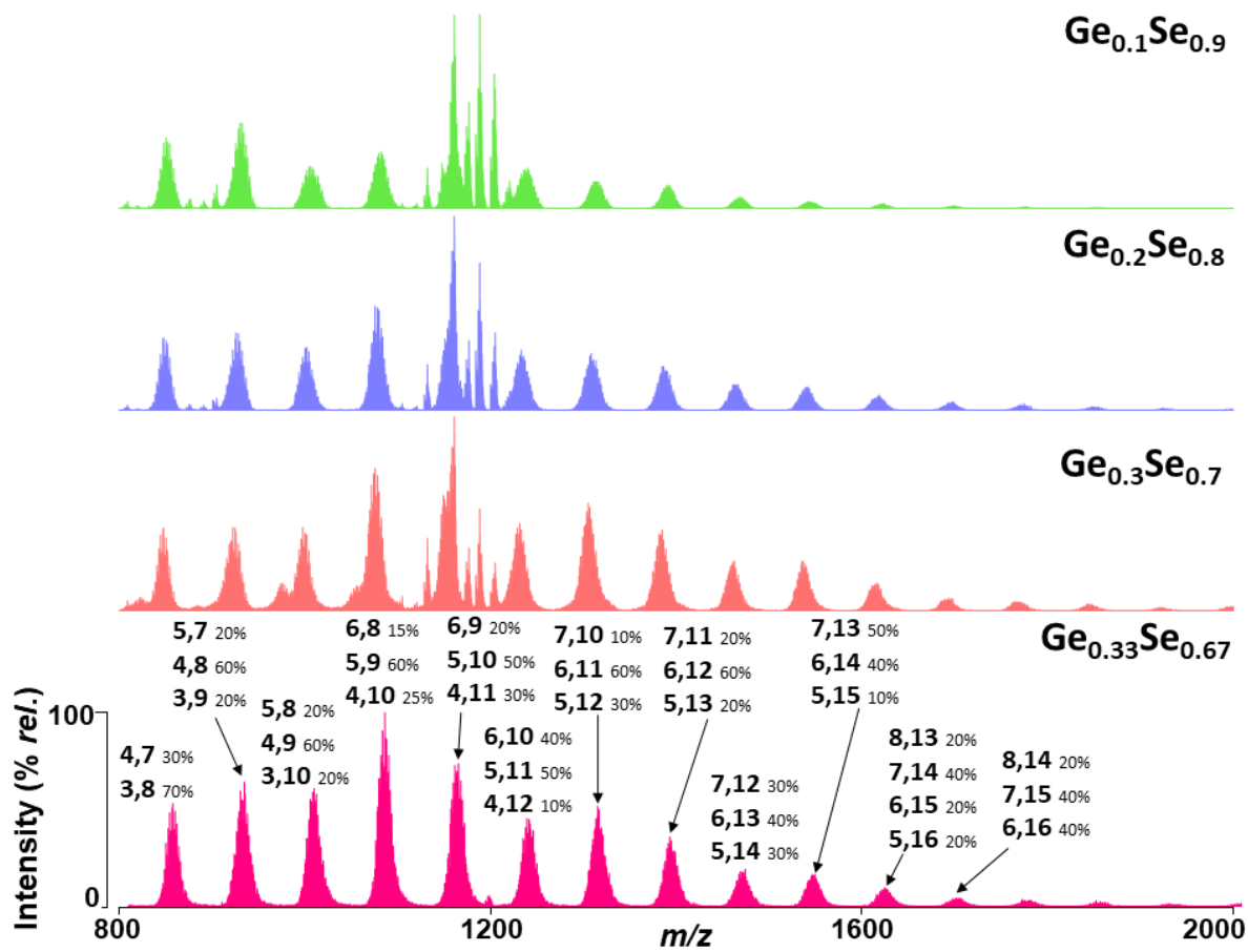
Fig. 2: Comparison of mass spectra obtained from all four bulk glass samples.
