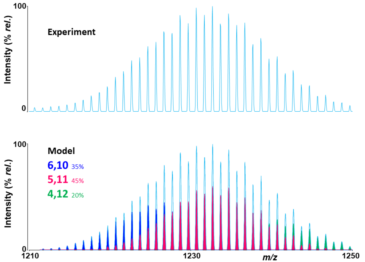
Fig. 3: Comparison of experimental and theoretical mass spectra obtained from \text{Ge}_{0.3}\text{Se}_{0.7} . Conditions: positive ion mode, laser energy 140 a.u.
