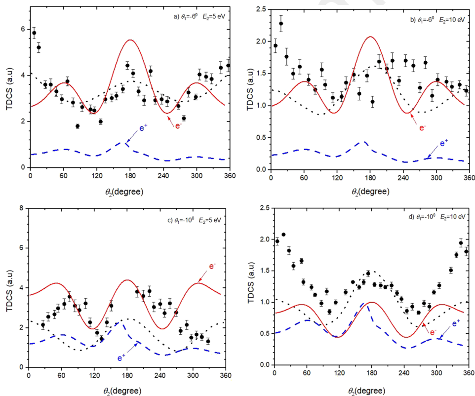
FIG. 2. Same as in Fig. 1 for the perpendicular geometry.
