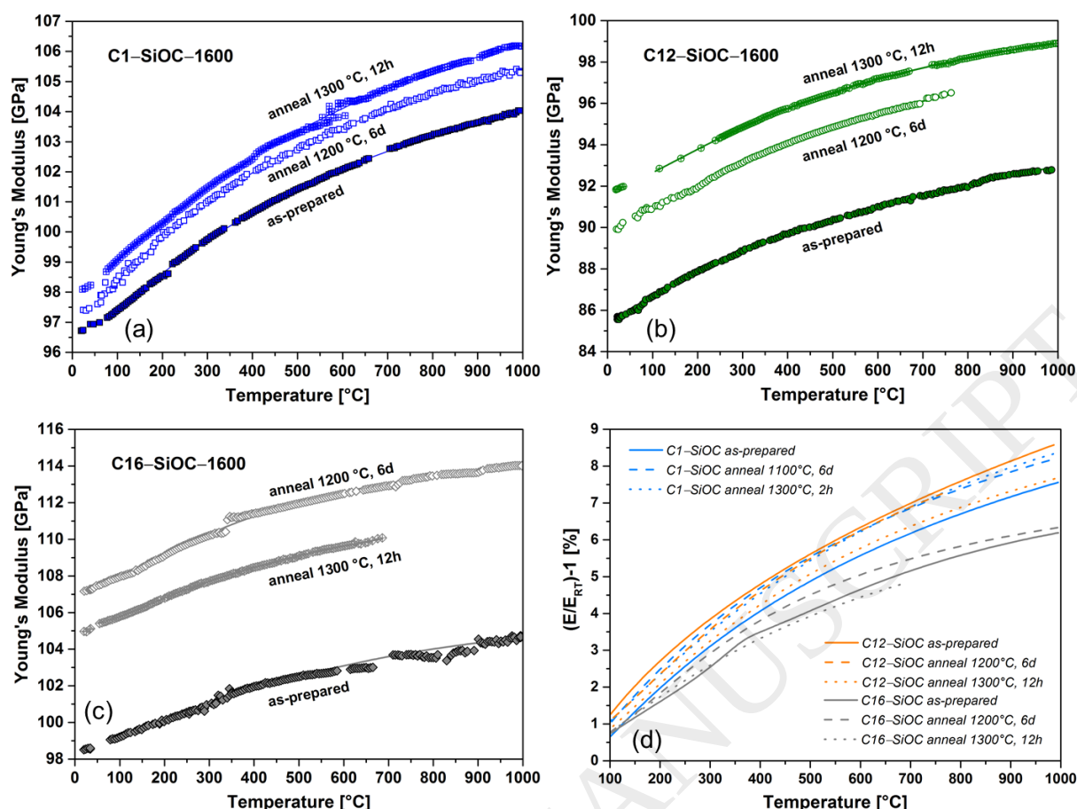
Figure 4. Temperature dependence of the Young's modulus of the as-prepared (a) C1-SiOC-1600 , (b) C12-SiOC-1600 and (c) C16-SiOC-1600 SiOC glass-ceramics, respectively, and after a thermal treatment at different temperatures and for varying durations. Lines drawn are fits to the experimental data. (d) Temperature dependence of the Young's modulus normalized to its value at room temperature (displayed by trendlines). The experimental error is estimated to be \pm 1 GPa (i.e., < 2 %).
