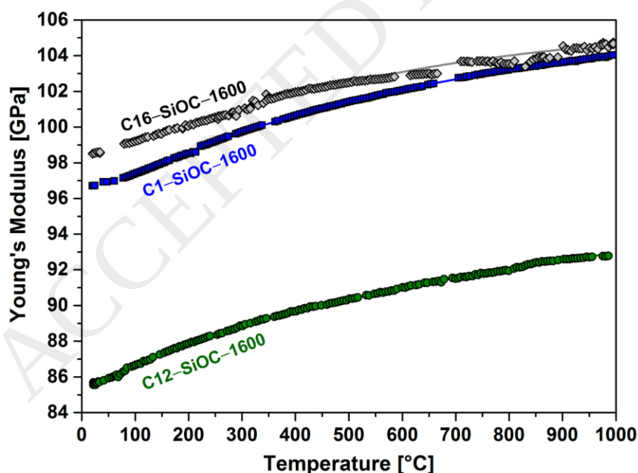
Figure 3. Temperature dependence of the Young's modulus of the SiOC glass-ceramics investigated in this study. The experimental error is estimated to be \pm 1 GPa (i.e., < 2\% ).
