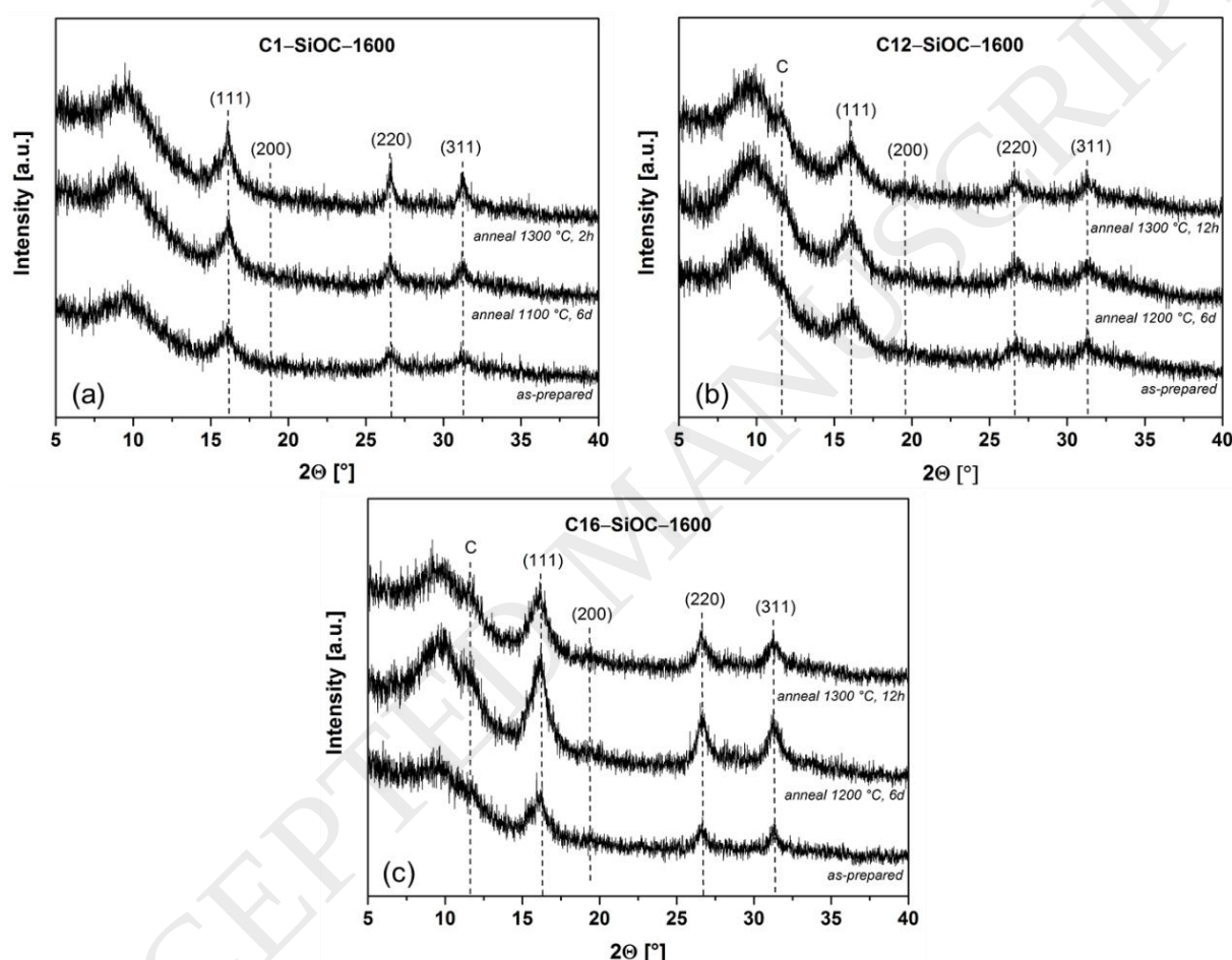
Figure 5. X-ray diffraction patterns (Mo K_\alpha ) of SiOC glass-ceramics prior and after annealing at high temperatures: (a) C1-SiOC-1600 ; (b) C12-SiOC-1600 ; (c) C16-SiOC-1600 . Indexed reflections relate to \beta -SiC.
