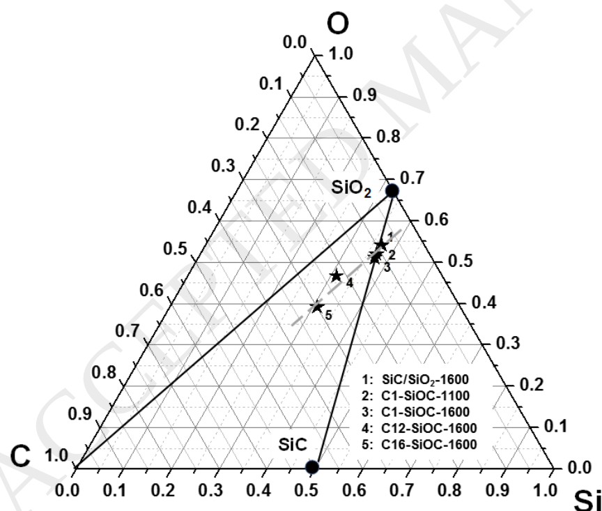
Figure 1. Ternary phase diagram in the system Si-O-C. The dashed line (parallel to the SiO 2 -C tie-line) marks that the segregated carbon content increases from SiC/SiO 2 -1600 to C16-SiOC-1600 without large variations in the SiC content.
