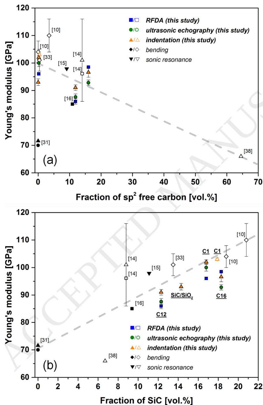
Figure 2. Room temperature Young's modulus of SiOC glasses (open symbols) and glass-ceramics (filled symbols) as a function of (a) volume fraction of sp^2 -hybridized segregated carbon and (b) the volume fraction of Si-C bonds (as for SiOC glasses) or \beta -SiC (as for SiOC glass-ceramics). Literature values (black symbols) are added for comparison. Dashed lines were drawn as a guide for the eyes.
