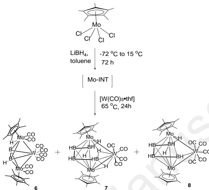
Scheme 3. Synthesis of diborene(2), ( 6 ) and heterometallaboranes ( 7 and 8 ). [Mo-INT] is an in situ generated intermediate, obtained from the reaction of [Cp*MoCl 4 ] and [LiBH 4 ] at -72 °C.
