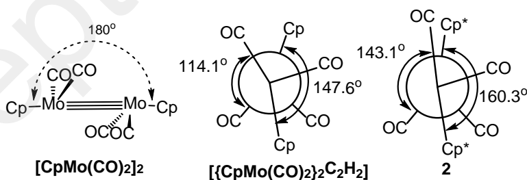
Chart 1. Schematic representation of the dihedral angles of Cp'...Mo-M...Cp' in [CpMo(CO) 2 ] 2 , [{CpMo(CO) 2 ] 2 C 2 H 2 ] and 2 (Cp' = Cp or Cp*).
