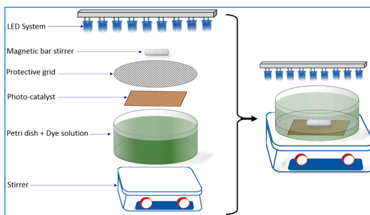
Figure 1. Photocatalytic apparatus for Reactive Green 12 (RG12) degradation.
