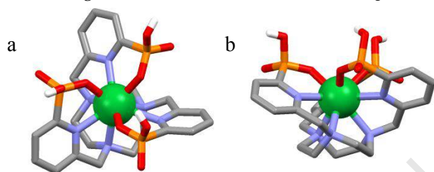
Figure 2. X-Ray crystal structure of the (YbL) complex viewed along (a) and perpendicularly (b) to the pseudo- C_3 axis.
