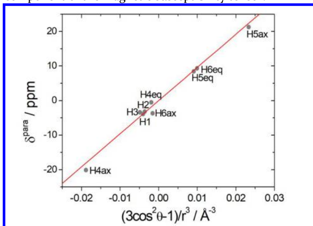
Figure 3. Plot of the paramagnetic shifts versus the geometric factors for the different proton nuclei of the \text{Yb}^{3+} complex. The red line corresponds to the linear fit of the data (See Scheme 1 for H atom labeling).
