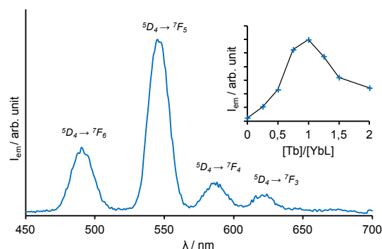
Figure 4. Emission spectrum measured upon addition of 1.0 equivalent of TbCl 3 ·6H 2 O to a 1.25 mM solution of (YbL) in D 2 O at pD 7.1 ( \lambda_{exc} = 980 nm, P_{980} = 1.08 W). Inset: Evolution of the emission intensity as a function of the [Tb]/[YbL] ratio.
