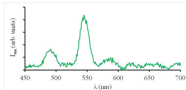
Figure 8. UC emission spectrum of an 11 mM solution of [YbL] in the presence of one equivalent of TbCl_3 \cdot 6H_2O upon excitation at 980 nm ( P_{980} = 1.08 W).
