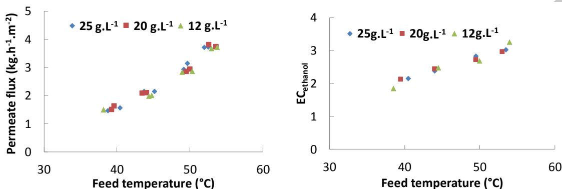
Figure 3: Influence of ethanol concentration and feed temperature on AGMD performance of water-ethanol binary mixtures: permeate flux (left) and EC ethanol (right) ( Q_{\text{feed}} = 5 \text{ L.min}^{-1} , Q_{\text{coolant}} = 4 \text{ L.min}^{-1} )
