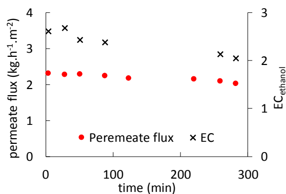
Figure 7: Time variation of the permeate flux and EC_{\text{ethanol}} (real algal-based fermentation broth, T_{\text{feed}} = 53^{\circ}\text{C} , Q_{\text{feed}} = 4.5 \text{ L}\cdot\text{min}^{-1} , Q_{\text{coolant}} = 4 \text{ L}\cdot\text{min}^{-1} )
