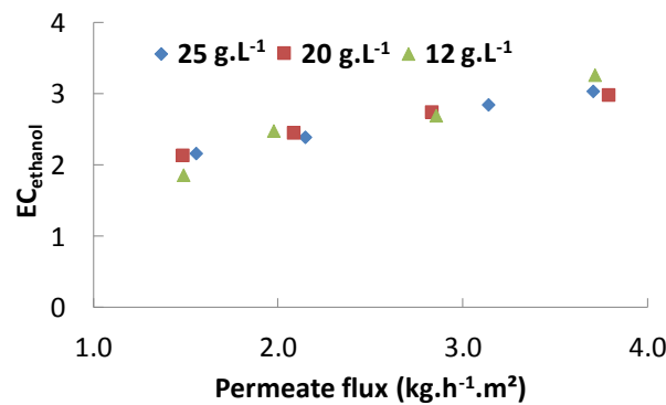
Figure 4: variation of EC_{\text{ethanol}} according to permeate flux for the water-ethanol binary mixtures
