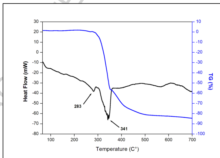
S.2: TG-DTA heating of [\text{Cd}_4\text{Cl}_{12}(\text{H}_2\text{O})_2]_n(\text{C}_{10}\text{N}_4\text{H}_{28})_n
