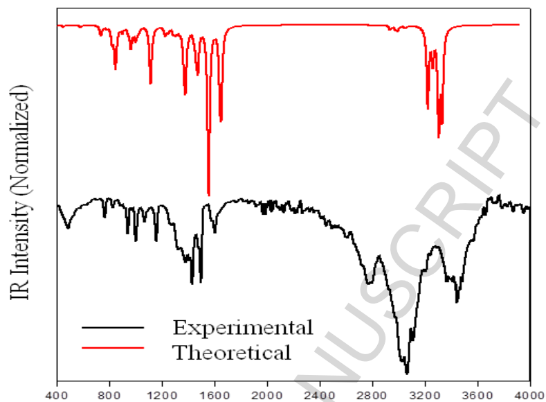
S.1: Simulated and experimental IR spectrum of [\text{Cd}_4\text{Cl}_{12}(\text{H}_2\text{O})_2]_n(\text{C}_{10}\text{N}_4\text{H}_{28})_n .
