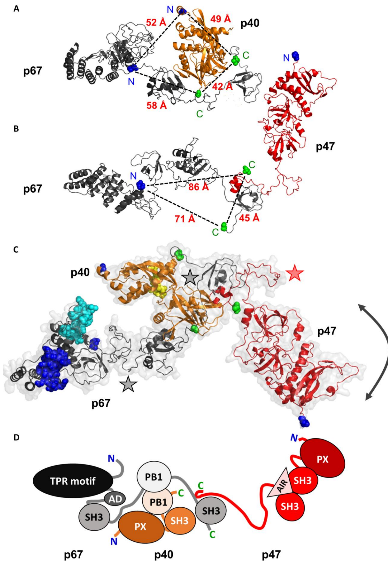
Figure 7. Proposed model of the complete cytosolic complex of phagocyte NADPH oxidase in the inactive state. Ribbon representation of p40^{\text{phox}} (orange), p47^{\text{phox}} (red), p67^{\text{phox}} (grey). The N-termini
