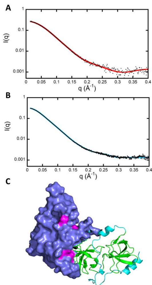
Figure 6. Modeling of p47 phox ΔCter from SAXS data. (A) Experimental SAXS curve measured on p47 phox ΔCter (black dots), compared to the calculated curve (red line) obtained from the selected model shown in (C) using the program CRY SOL ( \chi^2=0.97 ). (B) Experimental SAXS curve measured on full-length p47 phox (black dots) compared to the theoretical curve (blue line) calculated from the model of p47 phox shown in Fig. 7 ( \chi^2=1.25 ). (C) Selected SAXS model of p47 phox ΔCter that fulfills all the criteria discussed in the text and in Fig. S6. PX domain in violet, SH3 domains in green, AIR domain in cyan. Residues of the PX domain responsible for interaction with the membrane in the activated form are shown in pink.
