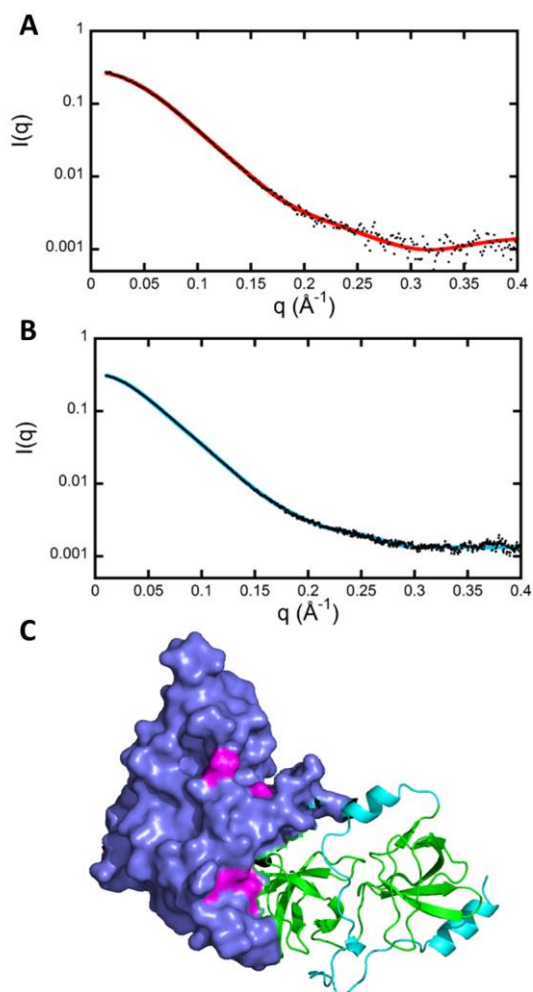
Figure 6. Modeling of p47 phox ΔCter from SAXS data. (A) Experimental SAXS curve measured on p47 phox ΔCter (black dots), compared to the calculated curve (red line) obtained from the selected model shown in (C) using the program CRY SOL ( \chi^2=0.97 ). (B) Experimental SAXS curve measured on full-length p47 phox (black dots) compared to the theoretical curve (blue line) calculated from the model of p47 phox shown in Fig. 7 ( \chi^2=1.25 ). (C) Selected SAXS model of p47 phox ΔCter that fulfills all the criteria discussed in the text and in Fig. S6. PX domain in violet, SH3 domains in green, AIR domain in cyan. Residues of the PX domain responsible for interaction with the membrane in the activated form are shown in pink.
