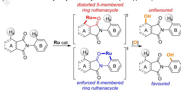
(C) Important ortho -hydroxy-substituted cyclic imides:
