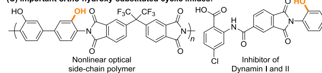
(C) Important ortho -hydroxy-substituted cyclic imides:
